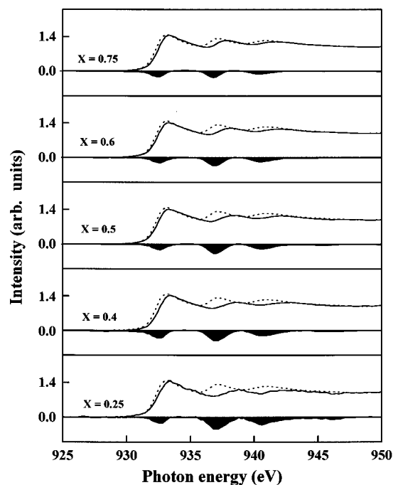
FIG. 5. Cu L_3 -edge difference curve between alloy (solid line) and Cu (dotted line); the area under the difference curve in the region of interest is darkened.
