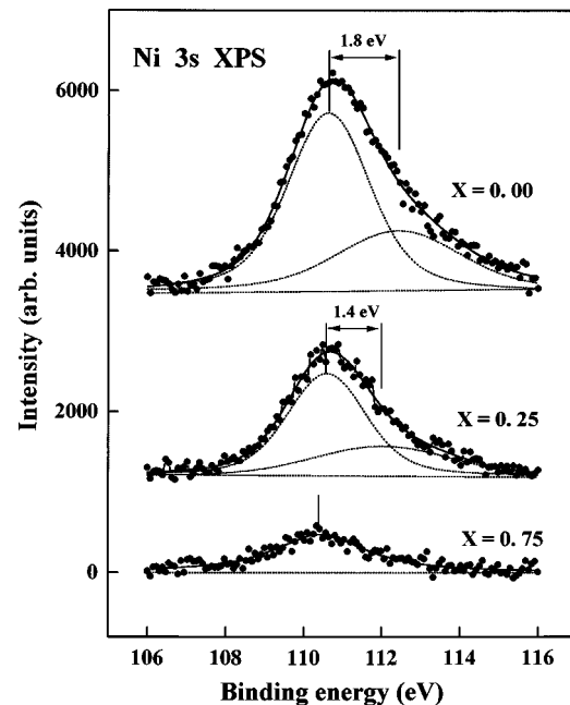
FIG. 9. The Ni 3s XPS spectra for some representative alloys. The final curves (solid line) were calculated by a summation of two individual peak curves shown by the dashed line. The experimental data were shown by the solid-circle line.
