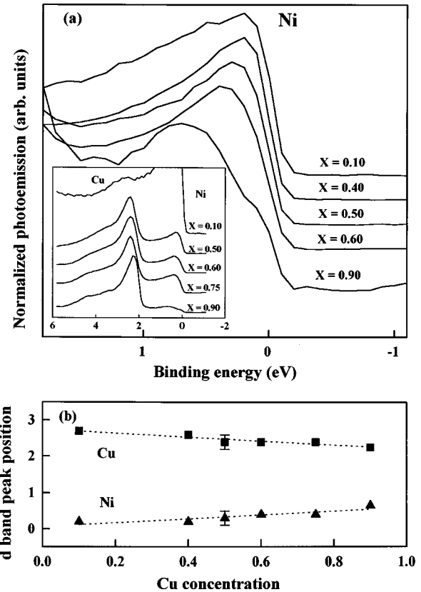
FIG. 1. (a) Representative Ni 3d valence-band spectra of Ni-Cu alloys. The inset presents the Cu 3d valence-band spectra. The intensities have been normalized to the maximum height of the bands. (b) A plot of Ni and Cu 3d binding-energy position vs Cu concentration x in alloys.
