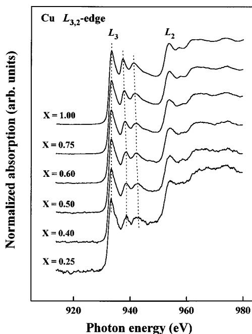
FIG. 3. Normalized Cu L_{3,2} -edge x-ray-absorption spectra of Ni-Cu alloys and pure Cu metal at room temperature.
