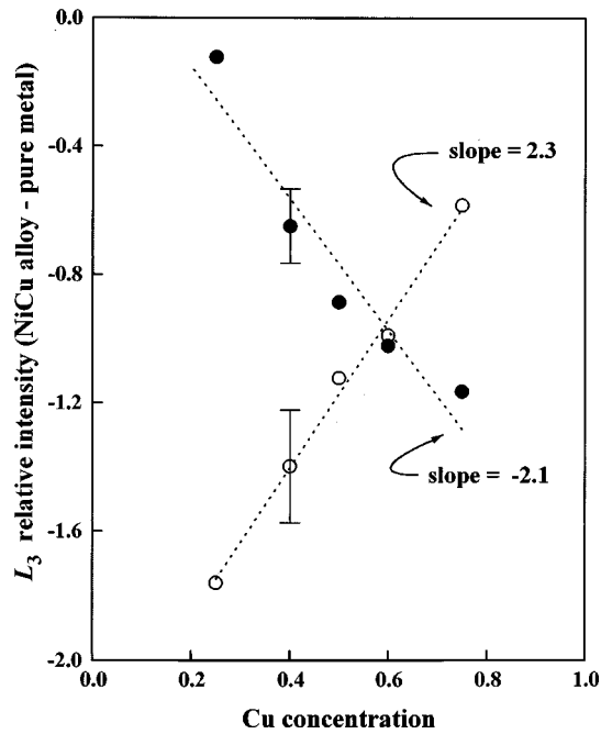
FIG. 6. Plot of difference curve intensity ( \Delta A ) vs Cu concentration x in alloys. The solid circle and open circle represent the \Delta A (Ni) and \Delta A (Cu), respectively. The dashed lines serve only as a visual guide for the \Delta A data.
