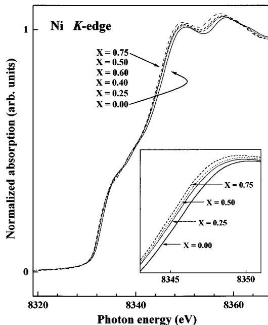
FIG. 7. Normalized Ni K -edge x-ray-absorption spectra of Ni-Cu alloys and pure Ni metal at room temperature. The region of threshold edge is inset on a magnified scale.
