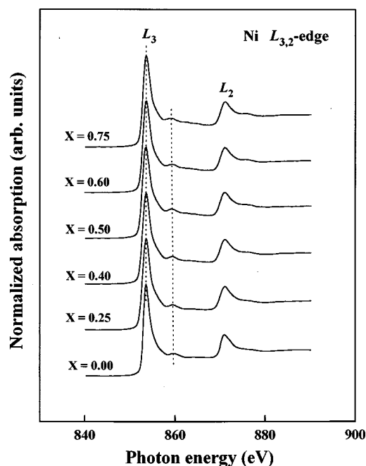
FIG. 2. Normalized Ni L_{3,2} -edge x-ray-absorption spectra of Ni-Cu alloys and pure Ni metal at room temperature.
