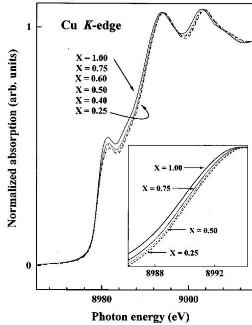
FIG. 8. Normalized Cu K -edge x-ray-absorption spectra of Ni-Cu alloys and pure Cu metal at room temperature. The region of threshold edge is inset on a magnified scale.
