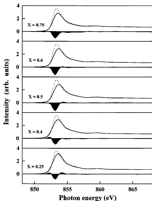
FIG. 4. Ni L_3 -edge difference curve between alloy (solid line) and Ni (dotted line); the area under the difference curve in the region of interest is darkened.
