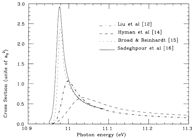
FIG. 3. Theoretical photodetachment partial cross section vs energy above the threshold for production of H(2) plus a free electron. Of the curves shown, the most recent calculation is that of Sadeghpour, Greene, and Cavagnero; the earliest is that of Hyman, Jacobs, and Burke.
