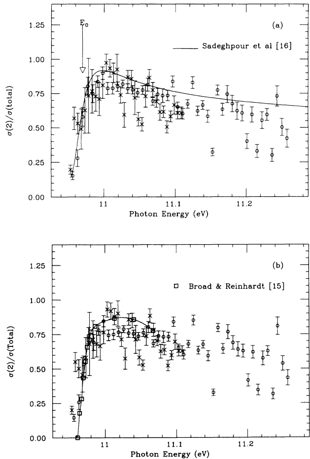
FIG. 6. Branching ratio vs photon energy for the H - ( n=2 ) shape resonance. The ratio was computed after binning the data into 7-meV bins. Error bars are statistical only. Open circles represent earlier data [6]. Crosses represent more-recent data [7]. (a) The solid line is the branching ratio prediction of Sadeghpour, Greene, and Cavagnero [16]. The arrow points to the approximate central energy position of the shape resonance. (b) The squares, indicating values computed from cross-section predictions of Broad and Reinhardt [15], are joined by a solid line to guide the eye.
