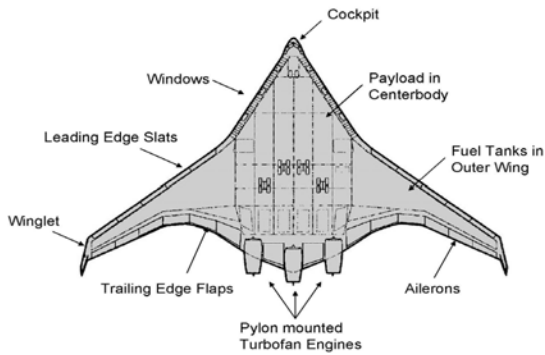
Figure 1. The Boeing BWB baseline. 7
