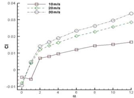
Figure 13. The rolling moment coefficient C_l vs. AOA at three different crosswinds.
