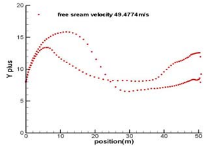
Figure 5. The Y plus distribution with free stream velocity 49.4774 m/s.
