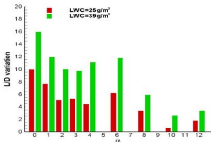
Figure 20. The lift to drag ratio vs. AOA comparison at two rain rates.
