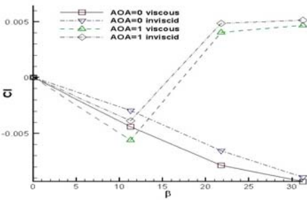
Figure 11. The rolling moment coefficient C_l vs. \beta at two different AOA.
