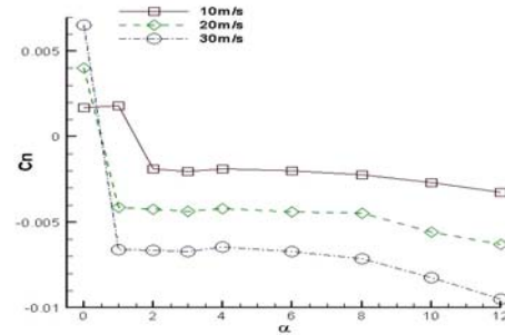
Figure 15. The yawing moment coefficient C_n vs. AOA at three different crosswinds.
