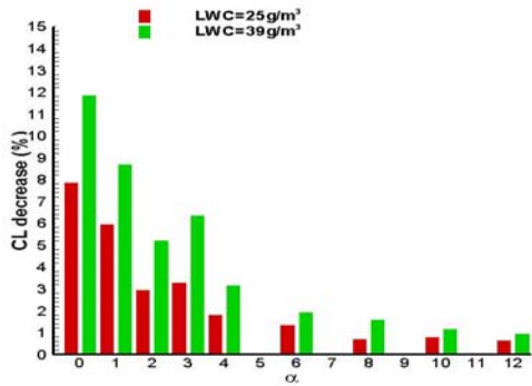
Figure 17. The lift coefficient decrease ratio at two different rain rates.
