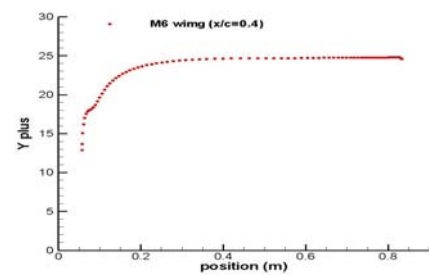
Figure 6. The Y plus of M6 wing at y/b=0.4 .
