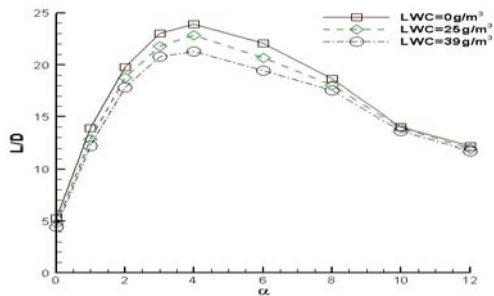
Figure 19. The lift to drag ratio vs. AOA at different rain rates.
