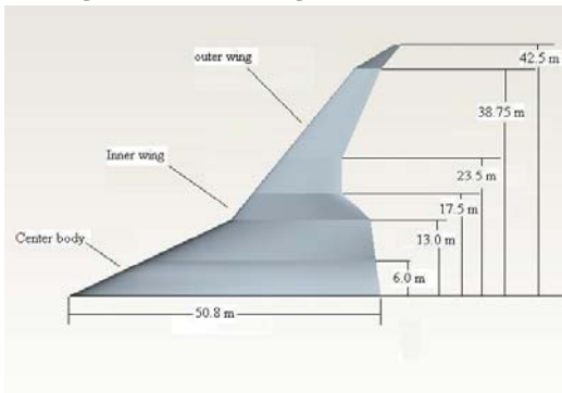
Figure 1. The Boeing BWB baseline. 7
