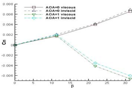
Figure 12. The yawing moment coefficient C_n vs. \beta at two different AOA.
