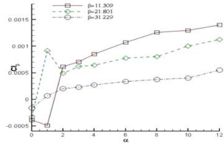
Figure 14. The stability derivative C_{l_\beta} vs. AOA at three different \beta .
