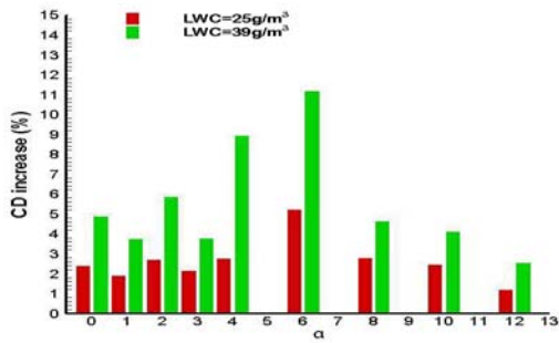
Figure 18. The drag coefficient increase ratio at two different rain rates.
