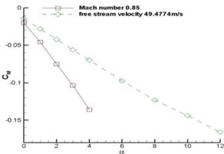
Figure 10. The pitching moment coefficient C_m vs. AOA at two different velocities.
