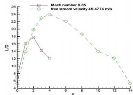
Figure 8. BWB lift to drag ratio vs. AOA at two different speeds.
