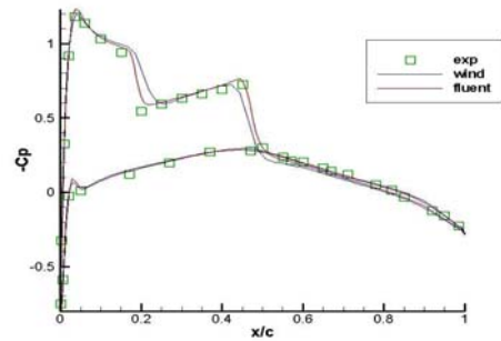
Figure 7. M6 C_p distribution at section y/b=0.65 .
