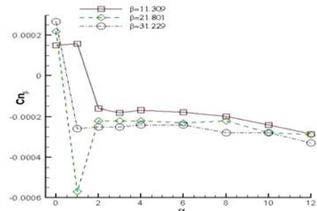
Figure 16. The stability derivative C_{n_\beta} vs. AOA at three different \beta .
