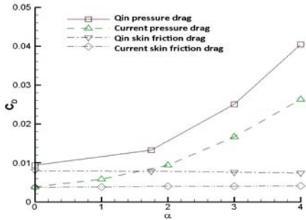
Figure 9. Pressure drag and skin friction drag comparison.
