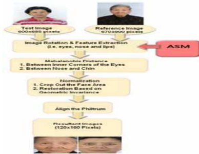
Figure. 2 Image normalization
