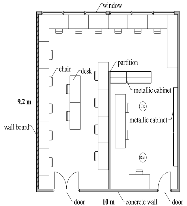
Fig. 3 A plan view of the simulated environment
