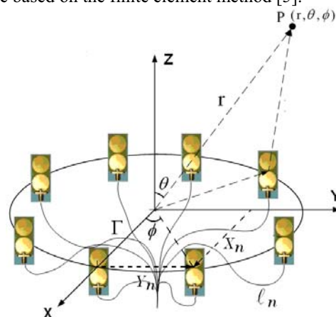
Fig. 1 Geometry of a circular antenna of 8 UWB printed dipole antennas
