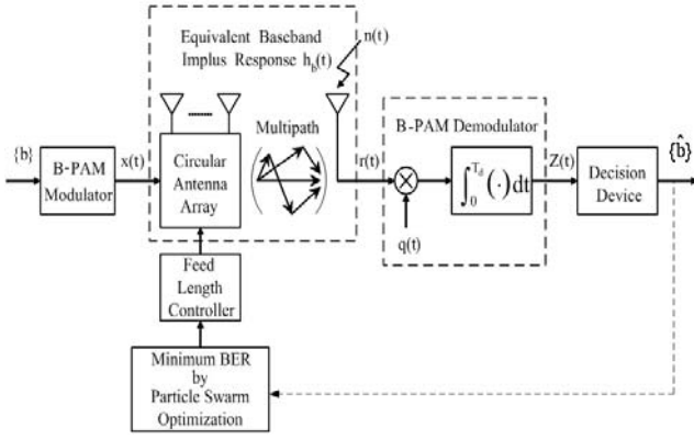
Fig. 2 Block diagram of the simulated system
