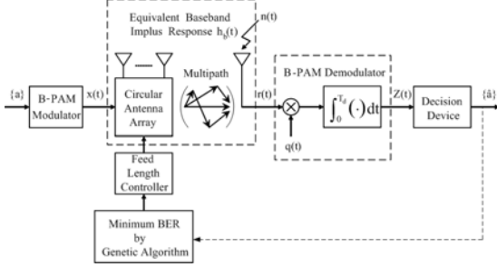
Figure 1. Block diagram of the simulated system
