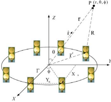
Figure 2. Geometry of a circular antenna of 8 UWB printed dipole antennas
