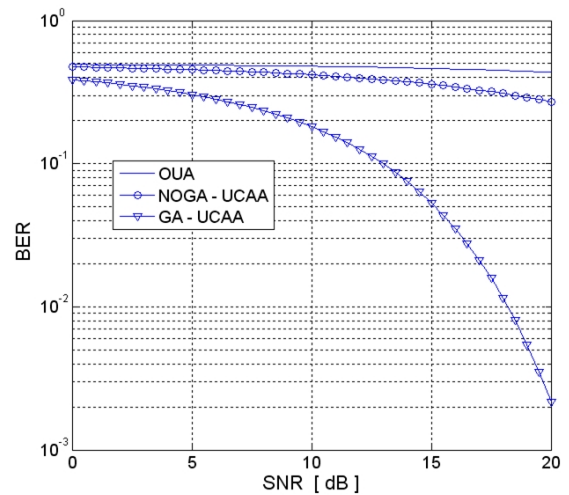
Figure 4. BER V.S. SNR over Scenario for three kinds of transmitter
