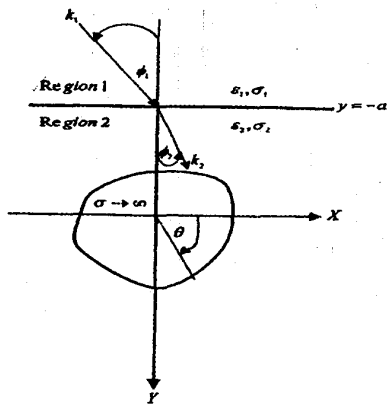
Fig. 1 Geometry of the problem in (x,y) plane
