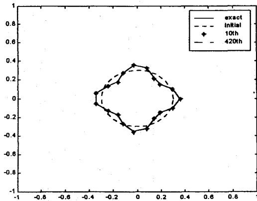
Fig. 3(a) Shape function. The solid curve represents the exact shape, while the dashed curves are calculated shape in iteration process. (b) Shape function error and conductivity error
