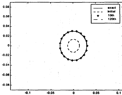
Fig. 4(a) Shape function. (b) Shape function error and conductivity error.
