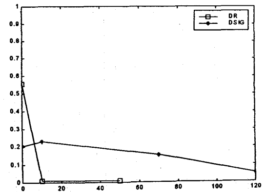
Fig. 3(a) Shape function. The solid curve represents the exact shape, while the dashed curves are calculated shape in iteration process. (b) Shape function error and conductivity error
