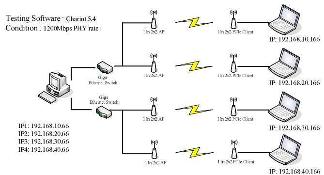
Fig. 2 System Structure of Multi-antenna Measurement System.
