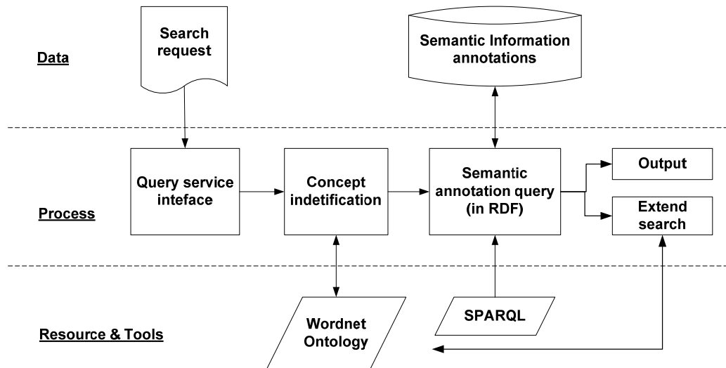
Figure 5. The flow of textual data retrieval using semantic annotations and Wordnet ontology.
