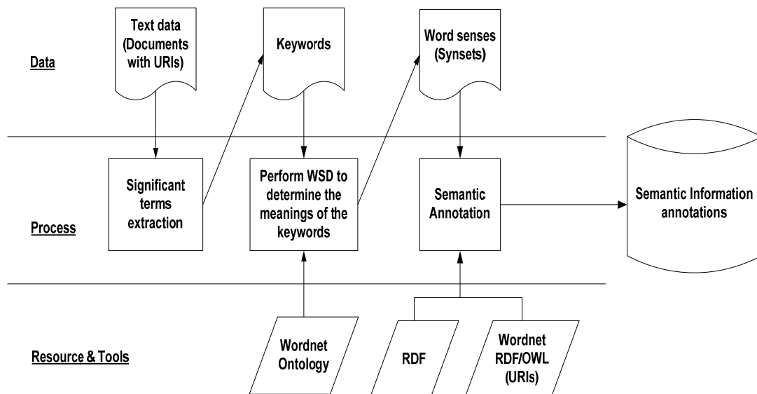
Figure 1. The process of annotating semantics to the textual data.
