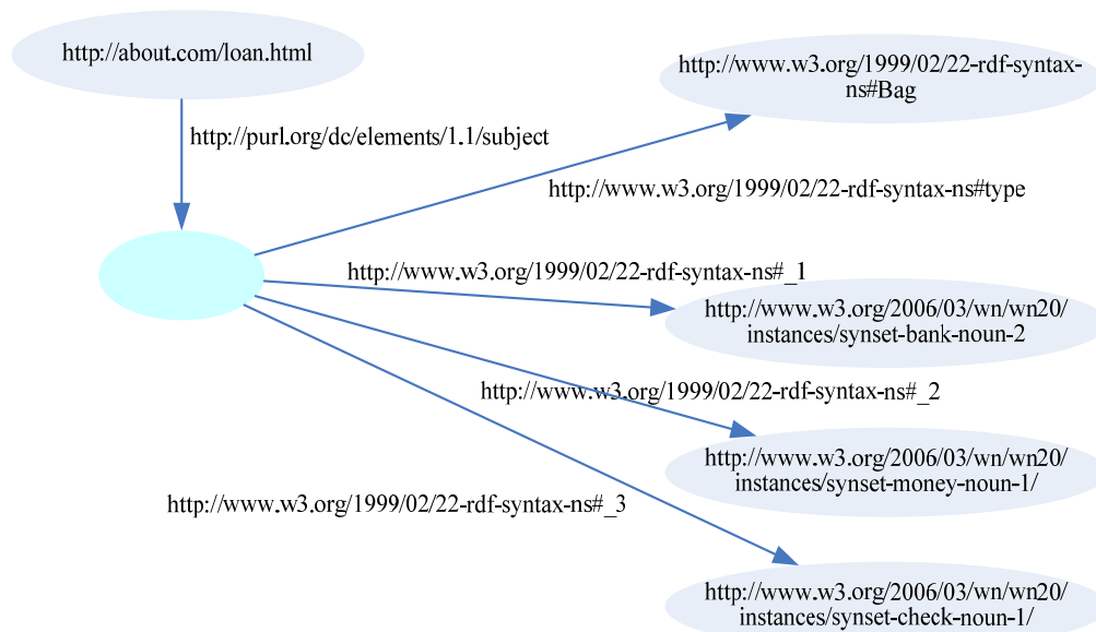
Figure 2. An example RDF graph indicating a document refers to three concepts.
