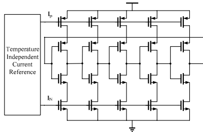
Fig. 4 Structure of CMOS ring oscillator with current-starved inverter stages
