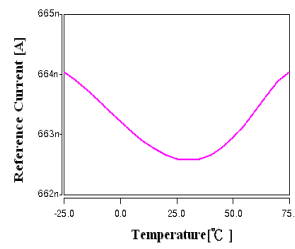
Fig. 5 Simulation plot of Fig. 1
