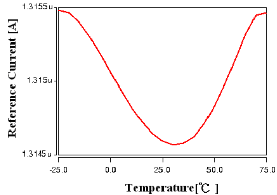
Fig. 7 Combination of the two architectures simulation plot
