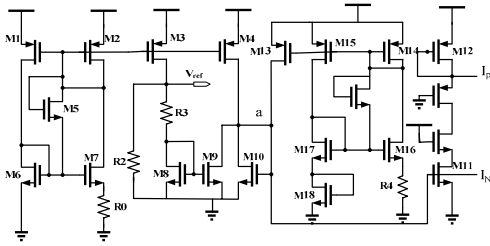
Fig. 3 Combination of the two architectures
