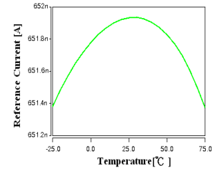
Fig. 6 Simulation plot of Fig. 2
