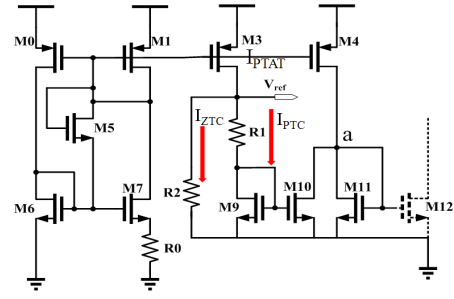
Fig. 1 Temperature compensation current reference
