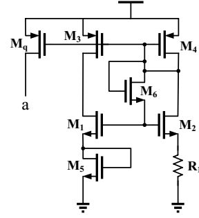
Fig. 1 Temperature compensation current reference
