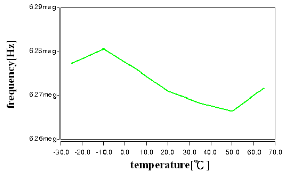
Fig. 8 The oscillation frequency versus temperature
