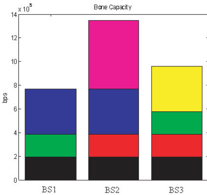
Figure 6. Bandwidth usage with coordination scheme implemented.
