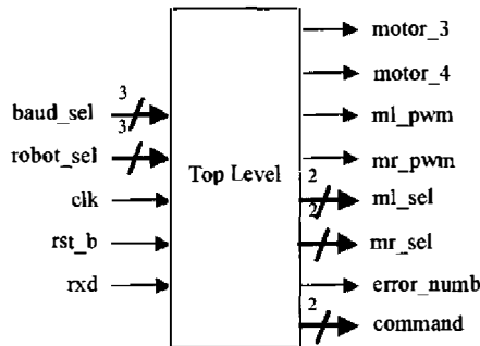
Fig. 1. I/O diagram of the proposed control IP for the soccer robot.
