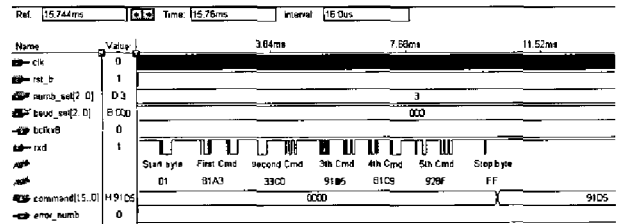
Fig. 12. The simulation diagram of the function data extraction.
