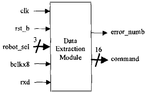
Fig. 5. Block diagram of the data extraction module.
