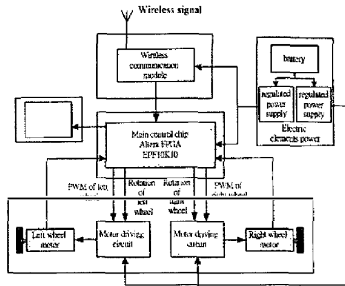
Fig. 9. The architecture of the soccer robot.
