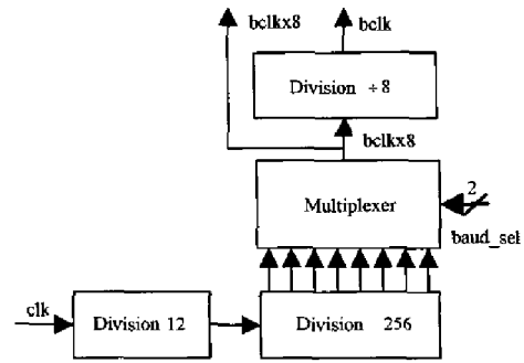
Fig. 2. Design diagram of the baud rate generation module.
