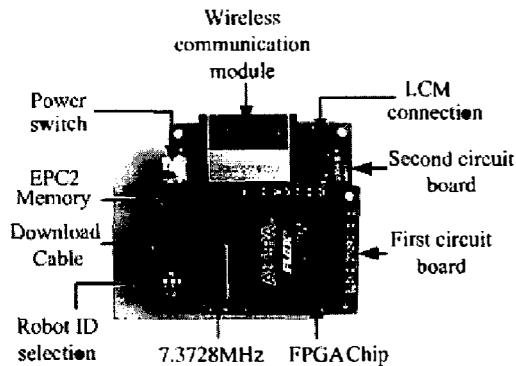
Fig. 10. The photograph of the control circuit board.
