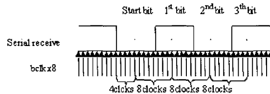
Fig. 3. Asynchronous serial data receiving method.
