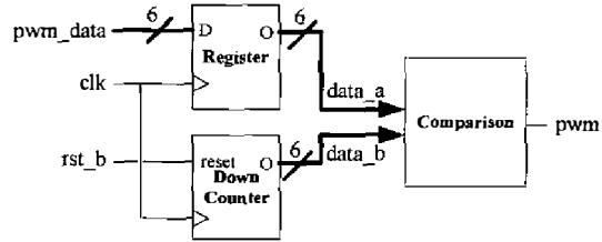
Fig. 7. Architecture diagram of the PWM signal generation module.
