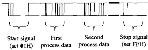
Fig. 4. Serial signals of the multi-control command
