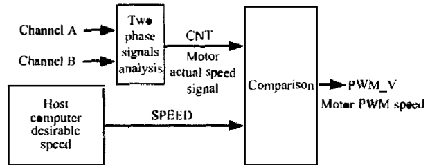
Fig. 8. Design flow diagram of motor feedback controller
