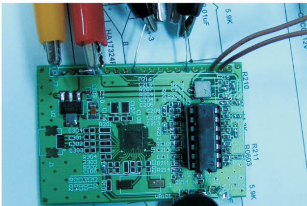
Figure 1. Test board of acceleration sensor.
