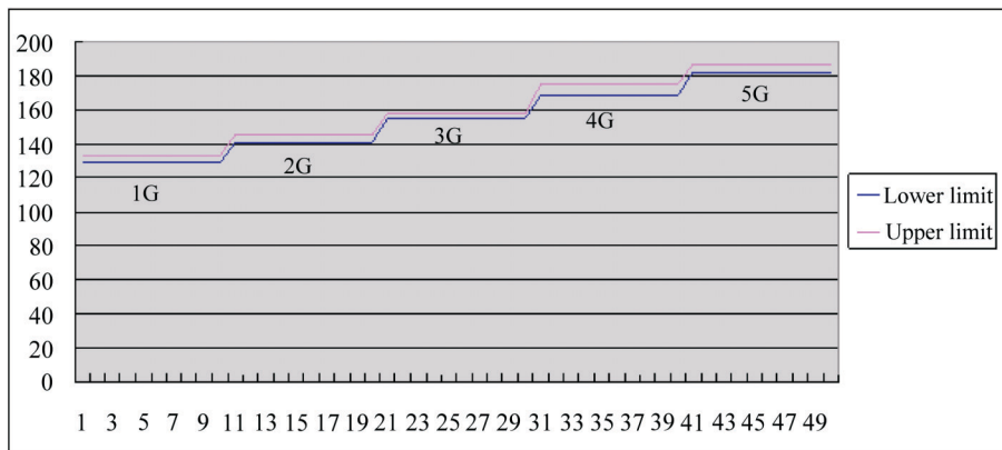
Figure 4. Data distribution resulting from 1G-5G vibrating force tests.
