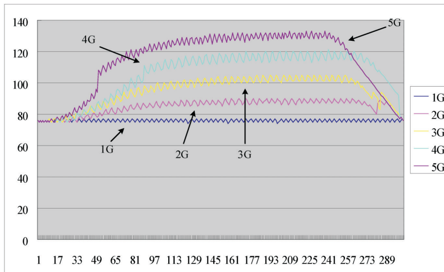
Figure 2. Test data in the x-axis.
