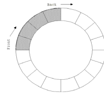
Figure 2. Ringed buffer
