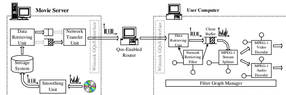
Figure 5. The system architecture for movie playback.
