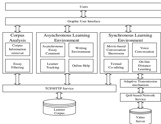
Figure 4. The system architecture of IWILL.
