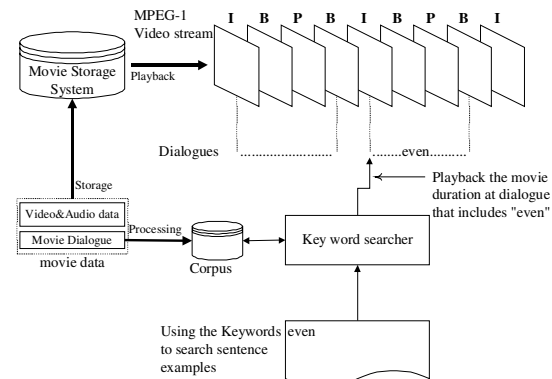
Figure 6. Movie processing for sentence searching.
