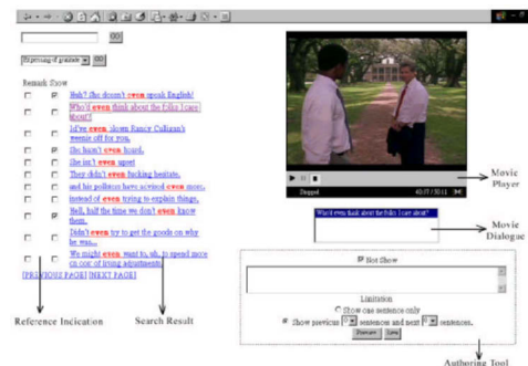
Figure 2. Teacher interface for mining English from movies.
