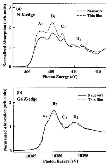
FIG. 2. (a) Normalized N K -edge and (b) Ga K -edge absorption spectra of GaN nanowires and thin film.
