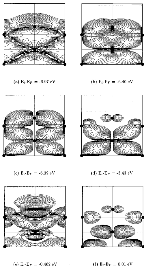
FIG. 4. Logarithmic partial charge density contour plots at \bar{\Gamma} for oxygen chemisorbed on the hollow site of Pt{100}-(1 \times 1), at the energies shown, at 0.5 ML. Cut along the (010) direction, through two directly bonded surface Pt atoms. The black dots show the atomic centers.
