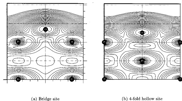
FIG. 3. Logarithmic total valence charge densities for oxygen chemisorbed on Pt{100}-(1×1). Cut along, (a) \langle 011 \rangle direction and (b) \langle 010 \rangle direction, through two directly bonded surface Pt atoms, and the O adatom, at a coverage of 0.5 ML.
