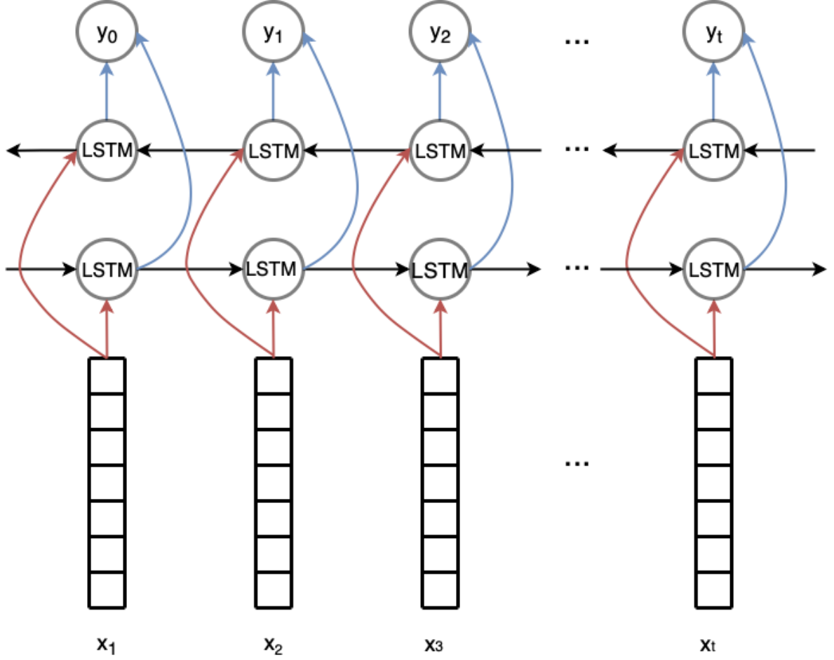
Figure 3.12: Bi-directional Long Short Term Memory Networks (biLSTM)
