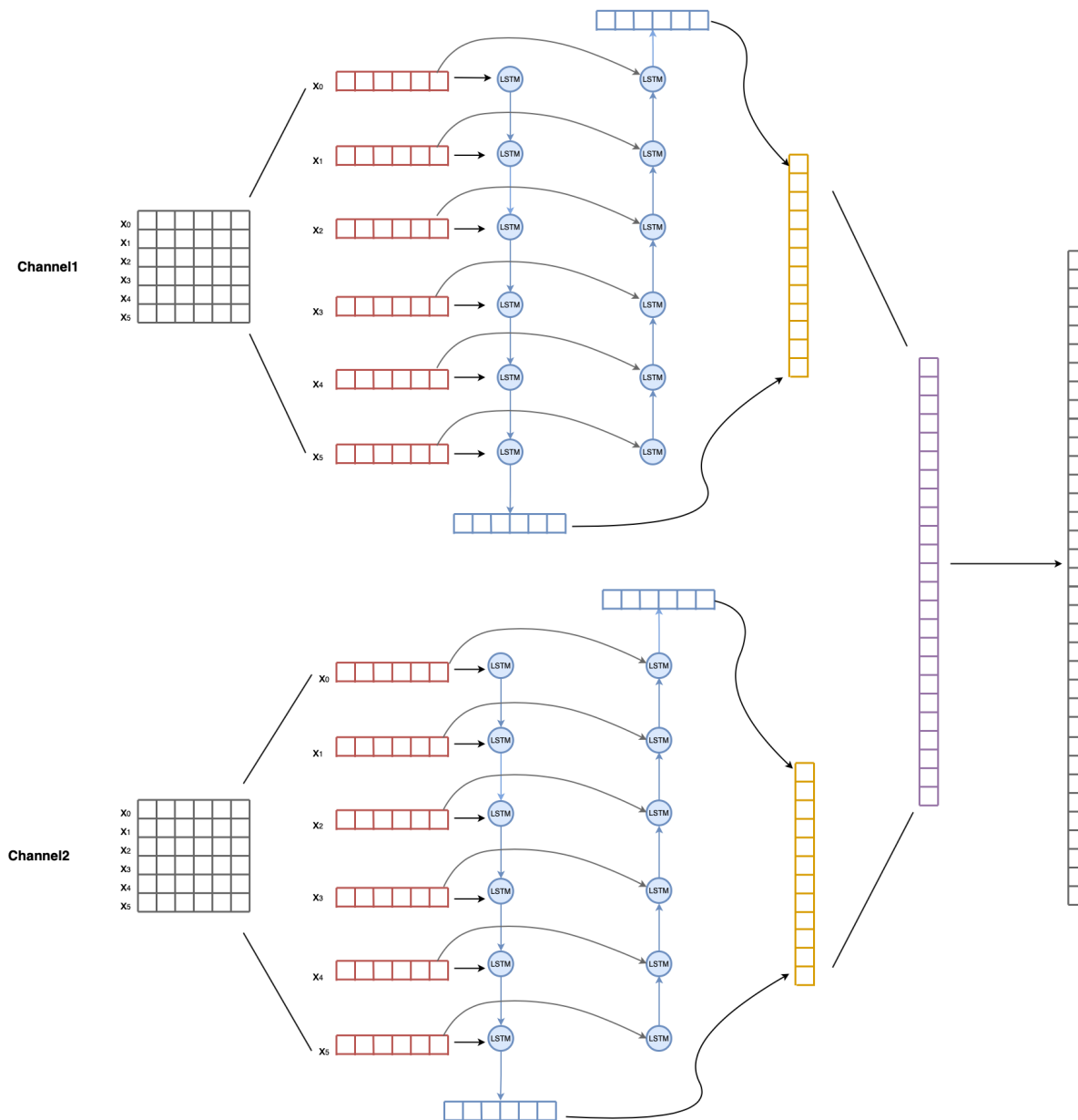
Figure 4.3: Multichannel biLSTM Architecture
