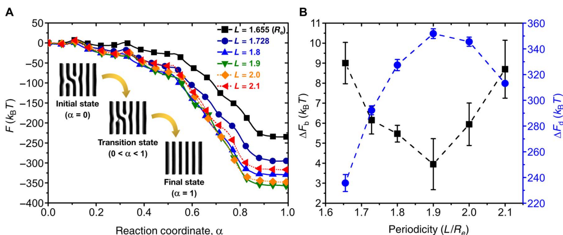
Fig. 4. MFEP calculation. (A) MFEPs between defective (dislocation dipole) and defect-free lamellar structures in symmetric BCP thin film at \chi N = 20 . The x axis represents the reaction coordinate \alpha along the pathway, while the y axis shows the free energy difference from the starting defective morphology, in units of k_B T . Morphologies of the initial defective ( \alpha = 0 ), transition, and final defect-free ( \alpha = 1 ) states are shown in insets. Periodicity, L , of lamellae varies from 1.655, 1.728, 1.8, 1.9, 2.0, to 2.1 R_e (end to end distance of polymer chain). The system size in lateral direction varies accordingly to L_x = 6L , while L_y and L_z are fixed at 8.275 and 1.655 R_e , respectively. (B) Defect formation energy, \Delta F_d (free energy difference between states at \alpha = 0 and \alpha = 1 , blue), and kinetic energy barrier, \Delta F_b (free energy difference between states at \alpha = 0 and the transition state, black), in units of k_B T , as a function of periodicity of lamellae. Each error bar shows the range from the average values.
