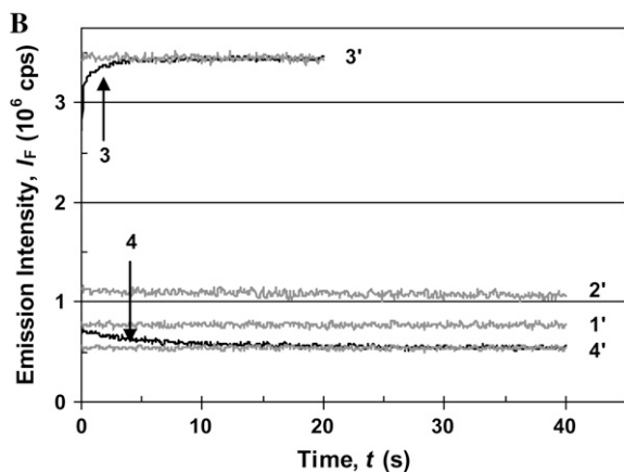
FIGURE 4 (A) Emission spectra of the main \beta -lactoglobulin conformations are: (1) native dimer in water, pH \approx 6 ( \beta_{\text{dim}} ); (2) native monomer in water, pH = 2.2 ( \beta_{\text{mon}} ); (3) state- \alpha , in DTAC micelles ( [\text{DTAC}] = 25 mM), pH \approx 6.5; and (4) state D, in 4 M GnHCl, pH \approx 6.5. (B) Unfolding kinetics of \beta -lactoglobulin with \lambda_{\text{exc}} = 293 nm and \lambda_{\text{em}} = 340 nm (curves in black) in 25 mM DTAC (3) and in 4 M GnHCl (4). The kinetic baselines obtained in the stopped-flow cell are shown for comparison (curves in gray): (1') in water, pH \approx 6.5, for the native dimer ( \beta_{\text{dim}} ); (2') in water, pH = 2.2, for the native monomer ( \beta_{\text{mon}} ); (3') in 25 mM DTAC, after stabilization of state \alpha ; and (4') in 4 M GnHCl, after stabilization of state D.
