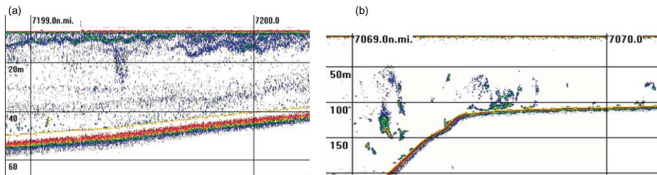
Figure 3. Typical acoustic recordings of horse mackerel by (a) night, and (b) day.
