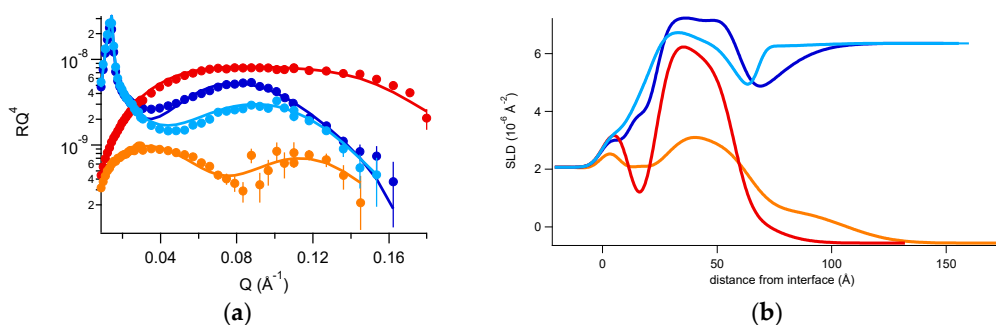
Figure 6. (a) Reflectivity curves (symbols), relative best fits (lines), and (b) obtained SLD profiles of the d_6 DPPC-GM1 membrane investigated in two contrasts before and after the deposition of the mucin layer on top of it. Color codes: red, membrane in H_2O NaCl; orange, membrane + mucin in H_2O NaCl; blue, membrane in D_2O NaCl; sky blue, membrane + mucin in D_2O NaCl.
