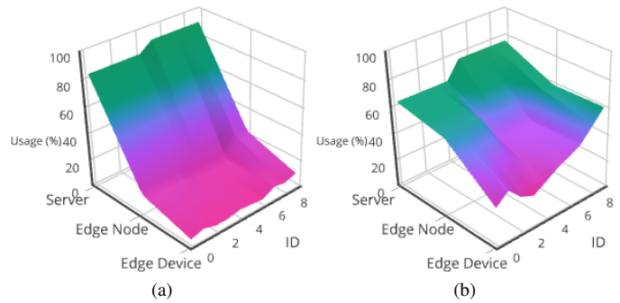
Fig. 8. Simulation results of load balance. (a)Edge devices directly upload the raw data for further process. (b) Edge devices and edge nodes participate in the pre-process of the captured data, using the proposed ECD model.
