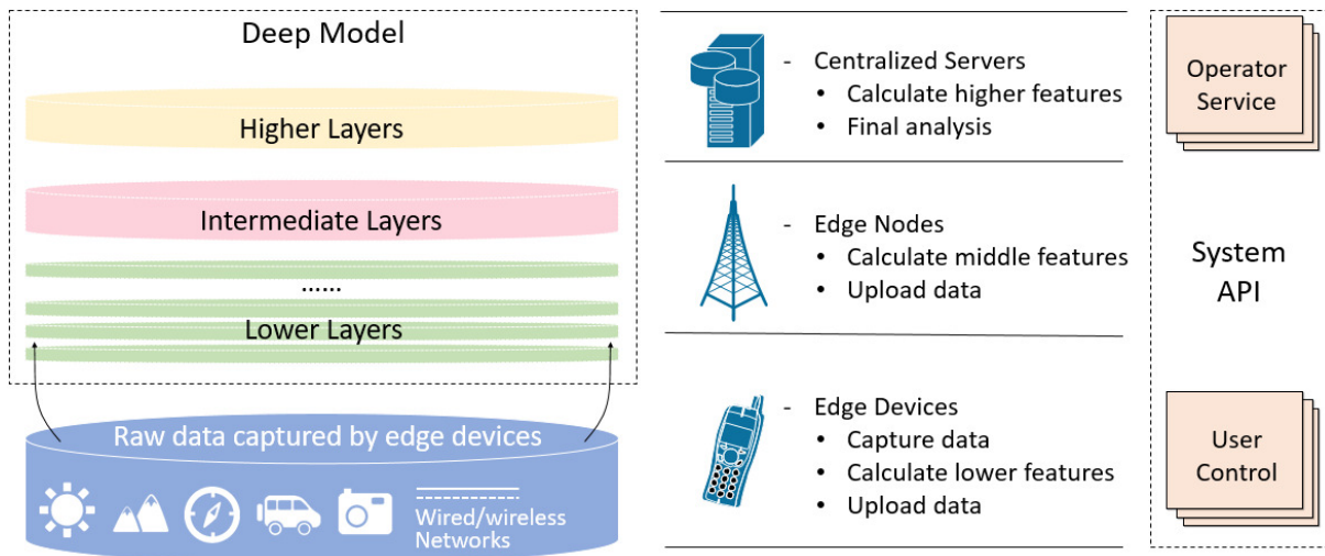
Fig. 2. The framework of the edge computing based deep learning system. The distributed deep model is allocated to all of the computing resource in the cloud, including centralized servers, edge nodes, and devices, for better load balance. Edge devices are responsible for the data sensing and lower layers calculation; the edge nodes calculate for the intermediate layers; the servers will perform the following higher layer calculation and final analysis. The crowdsensing process is fully controllable through some external APIs. Users can use the control panel to decide the balance between energy-saving and privacy protection.
