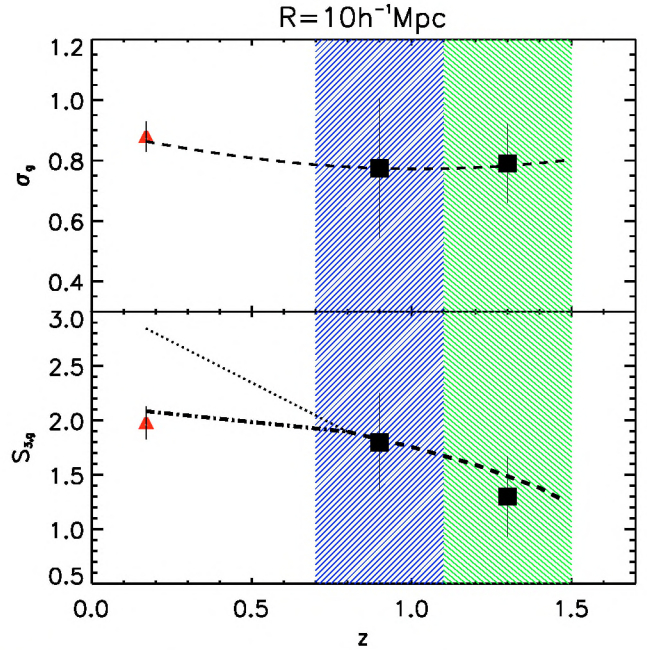
Fig. 4. Evolution of the rms deviation ( top ) and skewness ( bottom ) of the PDF of galaxy fluctuations on a scale R = 10 h^{-1} \text{ Mpc} . The filled squares correspond to two volume-limited samples from the VVDS with M_B < -20 + 5 \log h covering the redshift intervals indicated by the shaded regions. Triangles correspond to the 2dFGRS measurements at z \approx 0.15 (Croton et al. 2004), from a sample including similarly bright galaxies. Error bars give 68% confidence errors, and, in the case of VVDS measurements, include the contribution from cosmic variance. The dashed lines in both panels show the theoretical predictions for the evolution of the variance (Eq. (25)) and skewness (Eq. (27)) inferred using VVDS measurement of biasing. Predictions for the skewness (based on the (b_1(z), b_2(z)) measurements in the redshift range 0.7 < z < 1.5 quoted in Table 2 of Paper I) have been extrapolated to z \sim 0 using the local (2dFGRS) biasing measurements of Verde et al. (2002) (linear bias, dotted line) and of Gaztañaga et al. (2005) (quadratic bias with b_2/b_1 = -0.34 , dot-dashed line).
