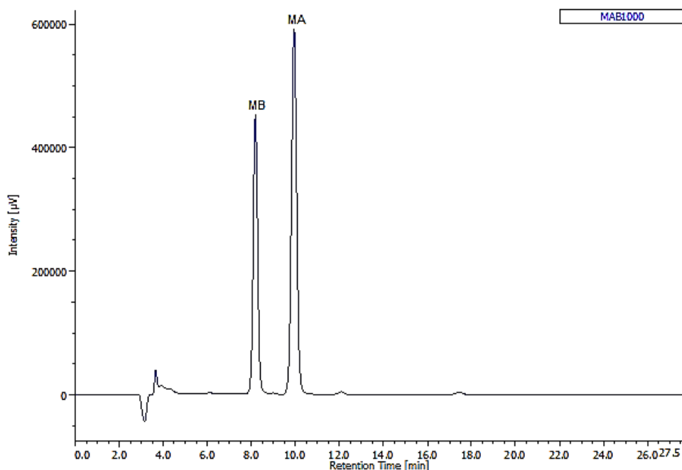
Figure 6. HPLC chromatogram of MA ( 10.01 \pm 0.04 min) and MB ( 8.22 \pm 0.03 min) measured at 210 nm.
