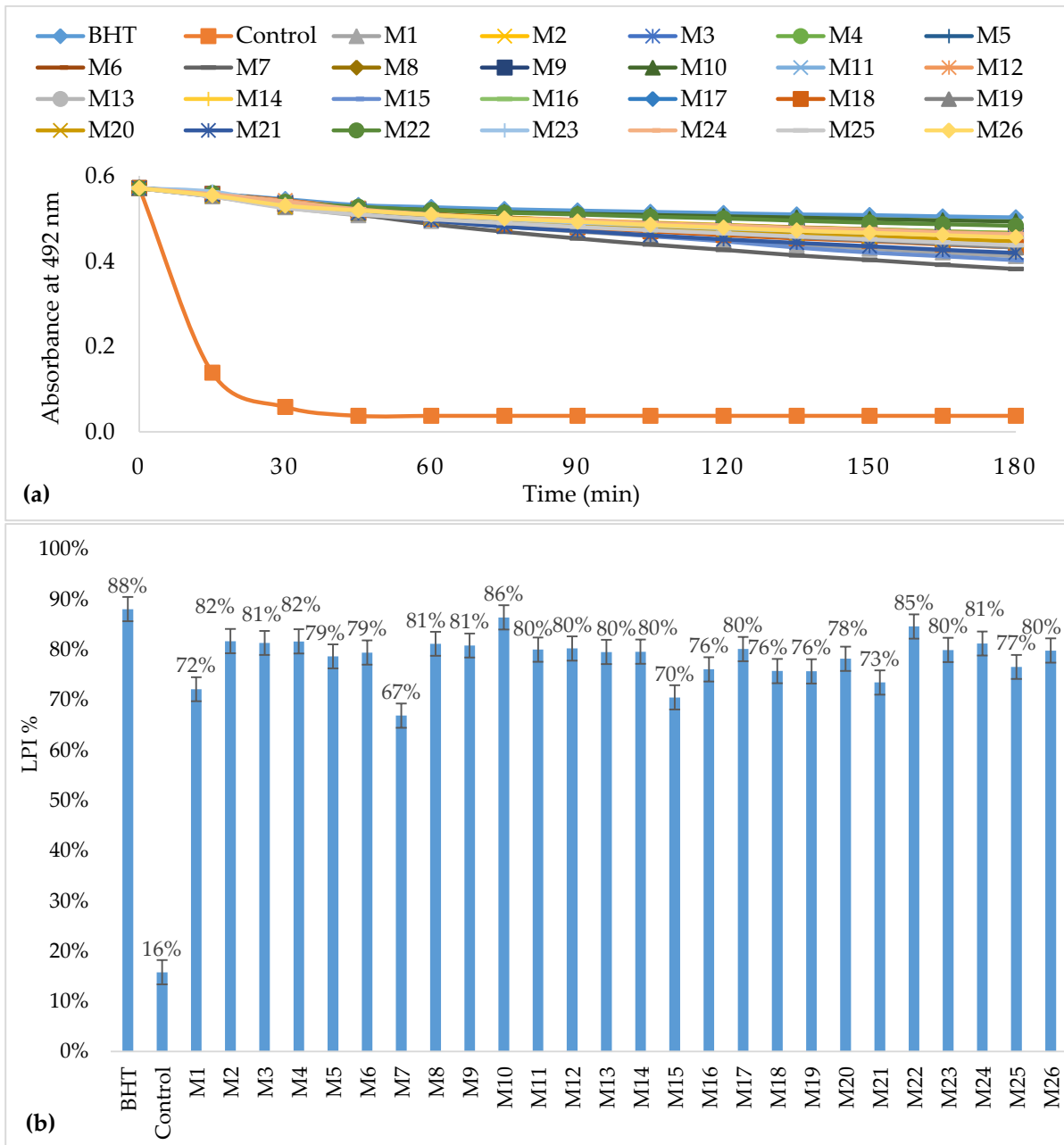
Figure 2. Antioxidant activities measured by \beta -carotene bleaching method (a) and their lipid peroxidation inhibition (%LPI) (b); Control (MeOH); BHT: butylated hydroxytoluene.
