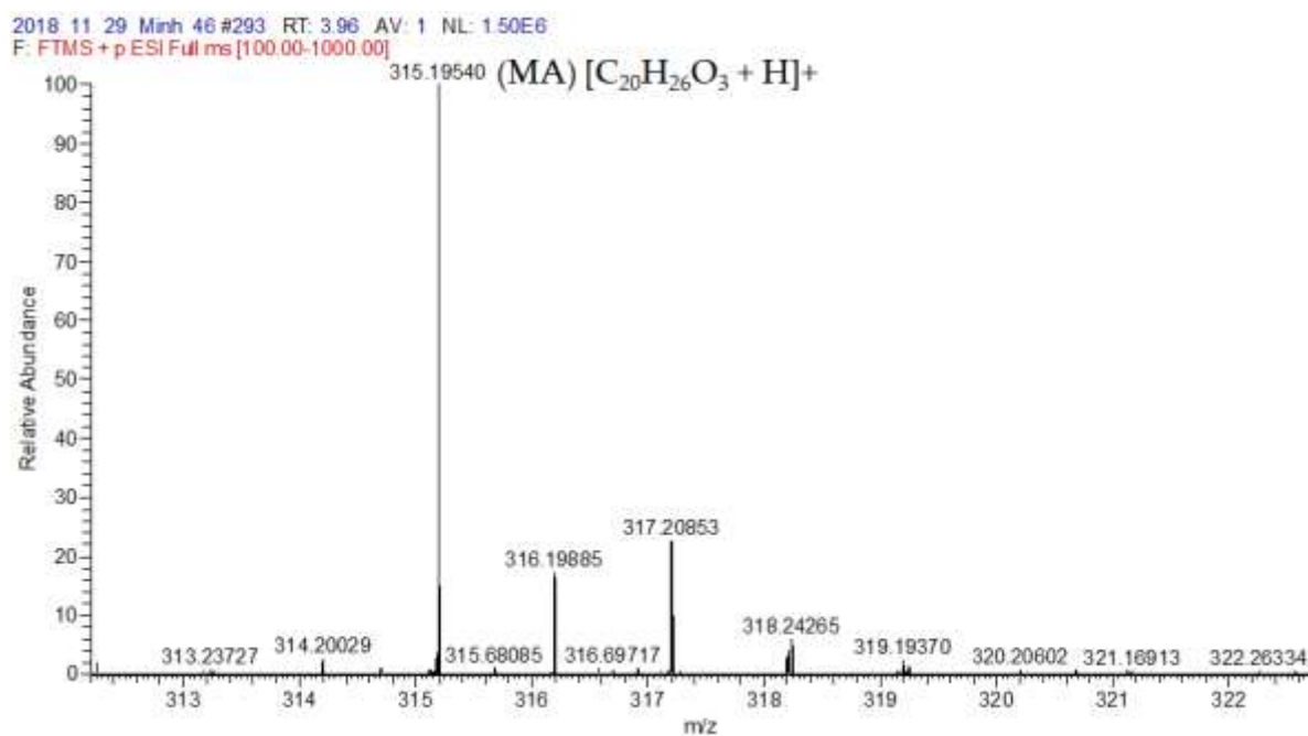
Figure S10a. UPLC/ESI-MS spectrum of MA detected in rice leaf essential oil.
