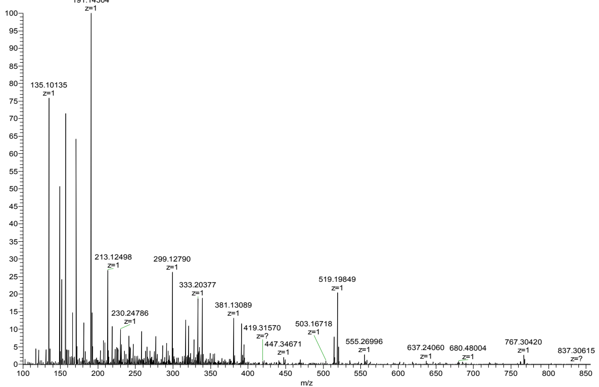
Figure S7a. ESI-MS spectrum of rice leaf essential oil.
