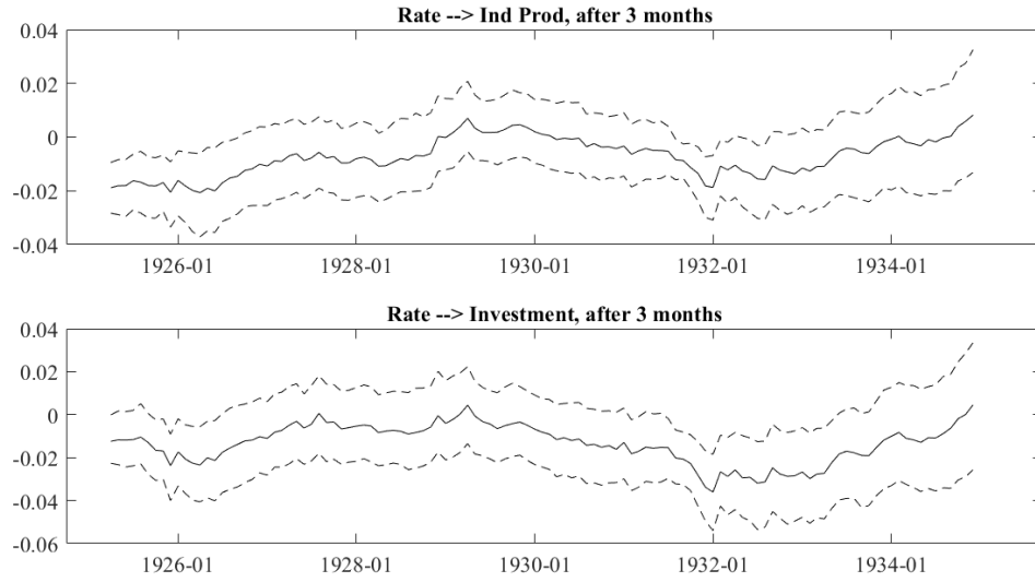
Figure 6: Impulse responses of industrial production and investment from interest rate shocks
