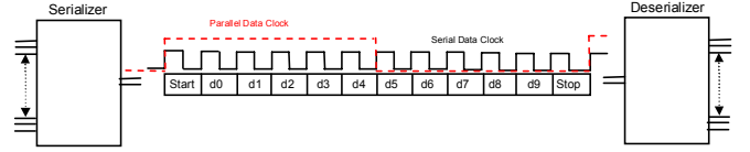
Figure 2. Clock embedded into serializer output.
