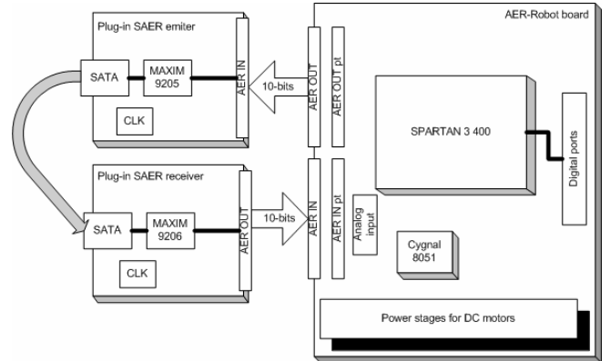
Figure 5. SAER link experiment block diagram
