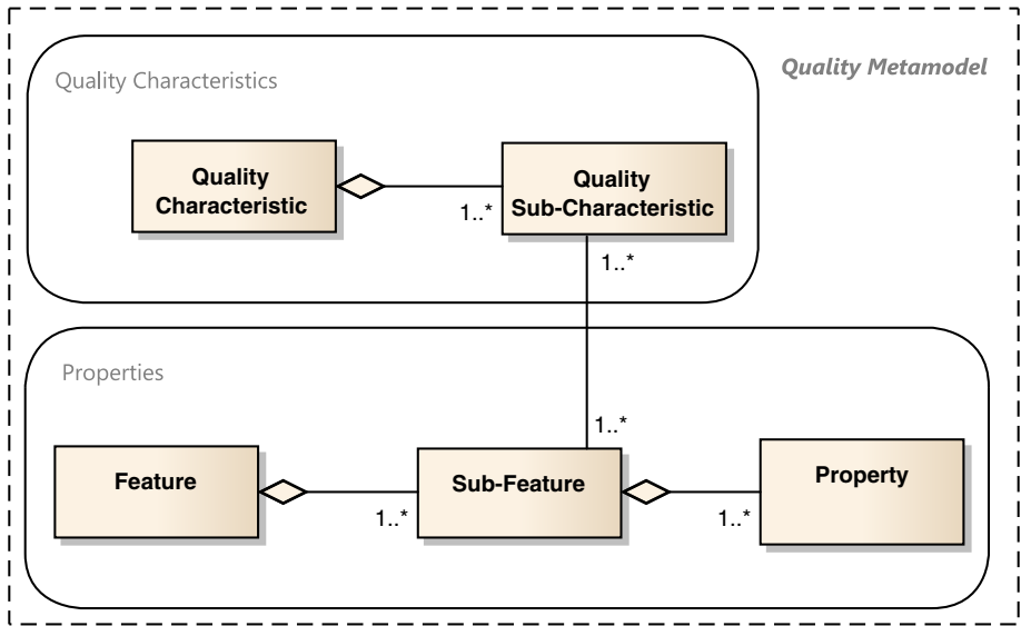
Fig. 2 Quality metamodel
