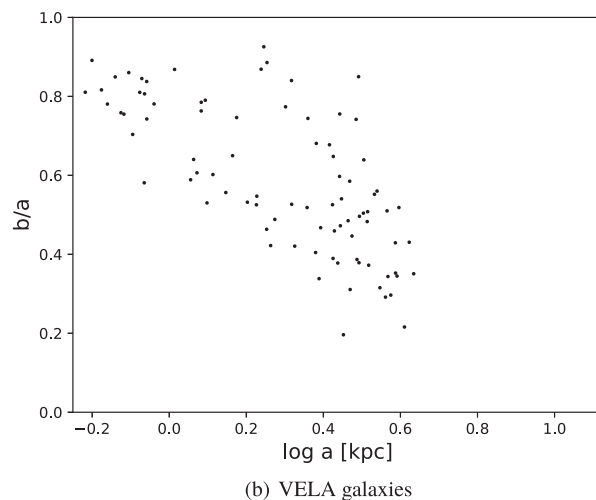
Figure 17. Panel (a): the b/a - \log a distribution of CANDELS star-forming galaxies in the early-prolate bin. Panel (b): The same distribution of elongated VELA galaxies in all mass-redshift bins. Elongated galaxies are defined as having a three-dimensional mass profile shape obtained by Tomassetti et al. (2016) that places them in the elongated region defined by Fig. 1. Only the truly random images as defined in Section 2.3 are plotted. There is an overall agreement between the model and observed distributions, but the VELA galaxies are on systematically rounder and larger in size than the CANDELS galaxies.
