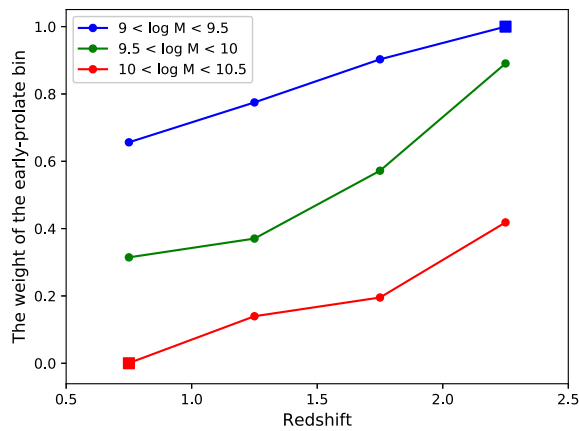
Figure 7. The evolving trend of the relative weight of the early-prolate bin with time and mass. The squares denote the cases in which the early-prolate or late-disky bins are themselves modelled, so the weight of the early-prolate bin is naturally unity or zero.
