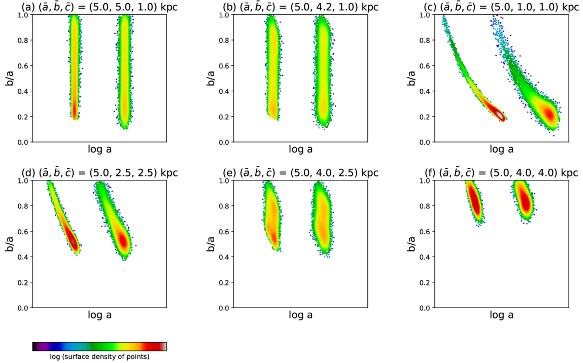
Figure 5. Comparison between b/a - \log a distributions of galaxies with different shapes, generated in the Sérsic modelling, and those generated in the ellipsoidal modelling. The one in the left of each panel is from the Sérsic modelling, and the other one in the right is from the ellipsoidal modelling. They are offset to the left and right for clarity. The points are colour coded by the number density of the points in their neighbourhood. The distributions generated by the two models are qualitatively the same, although they have different magnitudes of scatters.
