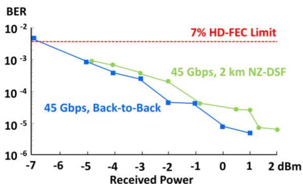
Figure 7. Received power vs. bit-error-rate showing error-free transmission for received power as low as -7 dBm.
