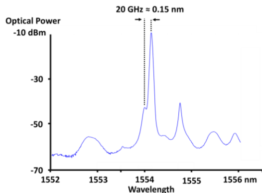
Figure 4. The filtered laser peak at the received side. The spacing between the main mode and the side mode is about 0.15 nm, which corresponds to 20 GHz.
