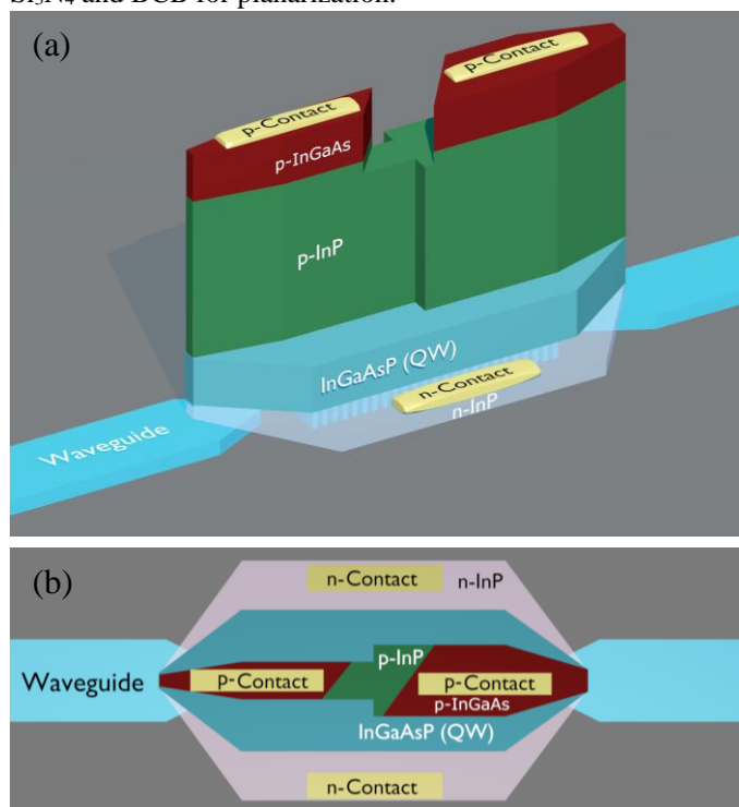
Figure 1. (a) 3D-view and (b) top-view of the fabricated InP-on-Si device showing electrically-isolated laser sections for independent current control.
