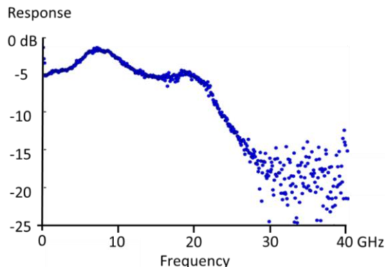
Figure 5. Small signal response showing nearly 25 GHz 3-dB modulation bandwidth at I_L = 46 mA and I_R = 60 mA.
