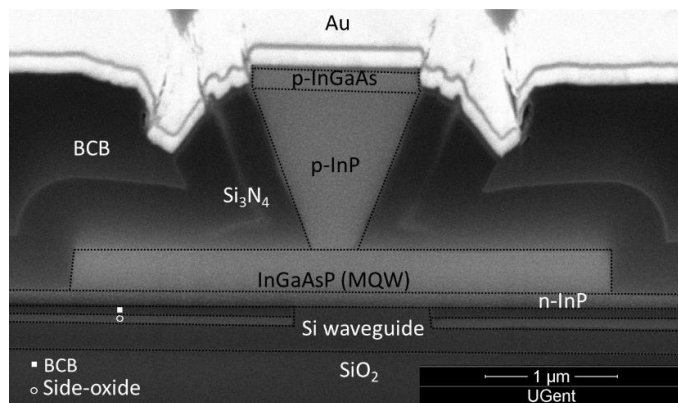
Figure 2. FIB cross-section image of a fabricated device showing the laser structure encapsulated in \text{Si}_3\text{N}_4 and BCB on top of a silicon waveguide.
