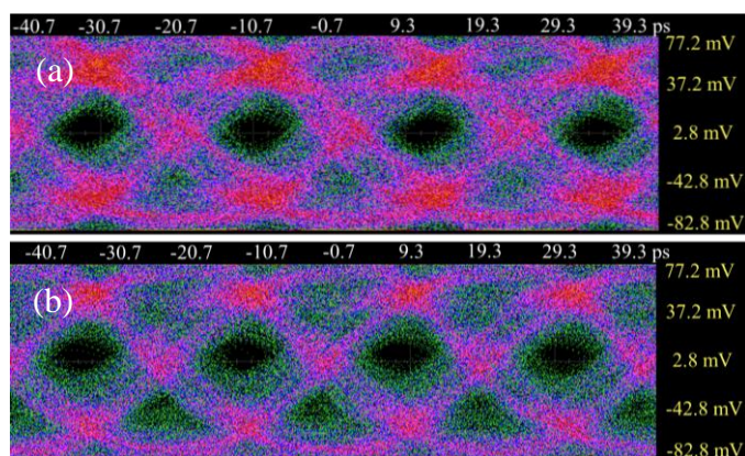
Figure 6. 45 Gbps error-free transmission showing (a) back-to-back and (b) with 2 km NZ-DSF, for a pattern length of 2^7-1 .
