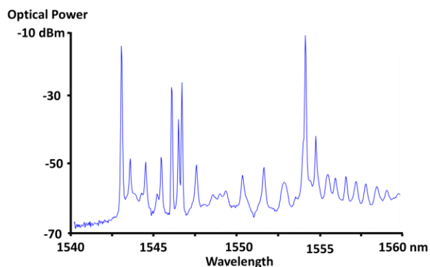
Figure 3. Optical spectrum of the laser at I_L = 48 mA and I_R = 60 mA. The right laser peak is filtered out at the receiver side.
