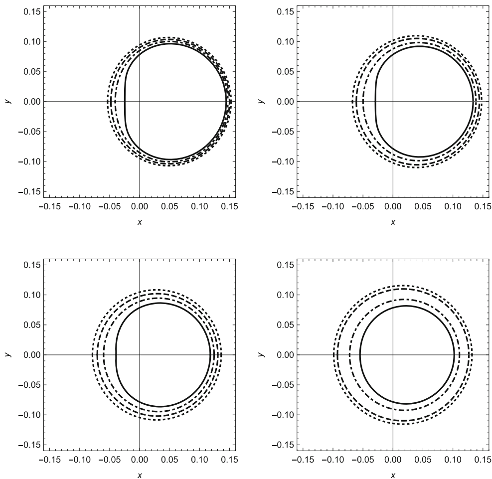
Fig. 1 Apparent shape of the black hole, as seen by an observer at r_0 = 50 and \theta_0 = \pi/2 , with \Lambda_{4D} = 10^{-7} , for different values of the rotation parameter a and the tidal charge q . Upper row, left: a = 0.83 , q = q_c \approx 0.30 (full line), q = 0.1 (dashed-dotted line), q = -0.1 (dashed line), and q = -0.3 (dotted line). Upper row, right: a = 0.7 , q = q_c \approx 0.51 (full line), q = 0.2 (dashed-dotted line),
