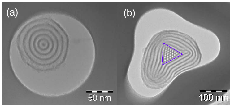
Figure 7. Top-view TEM images of mesoporous carbon nanofibres showing the influence of the size and shape of the AAO pores on the arrangement of the mesochannels.
