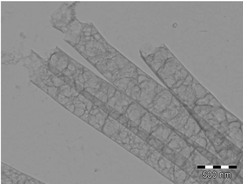
Figure 6. TEM image of carbon structures prepared by using CTAB as a structural directing agent.
