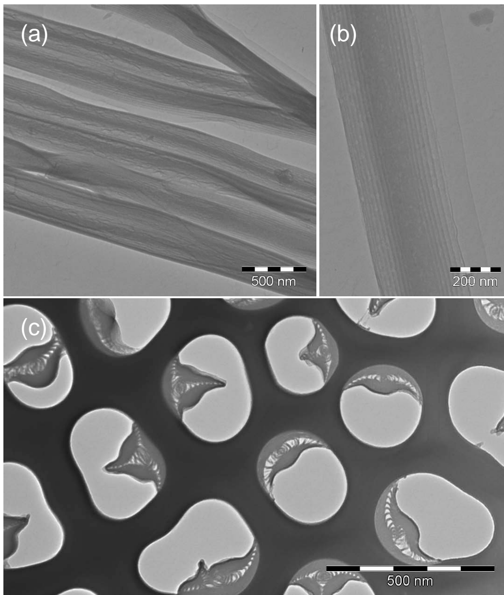
Figure 5. Side-view (a) and (b), and top-view (c) TEM images of mesoporous carbon nanoribbons prepared by using P123 as a structural directing agent, showing the circular mesochannels running parallel to the longitude axis of the ribbons.
