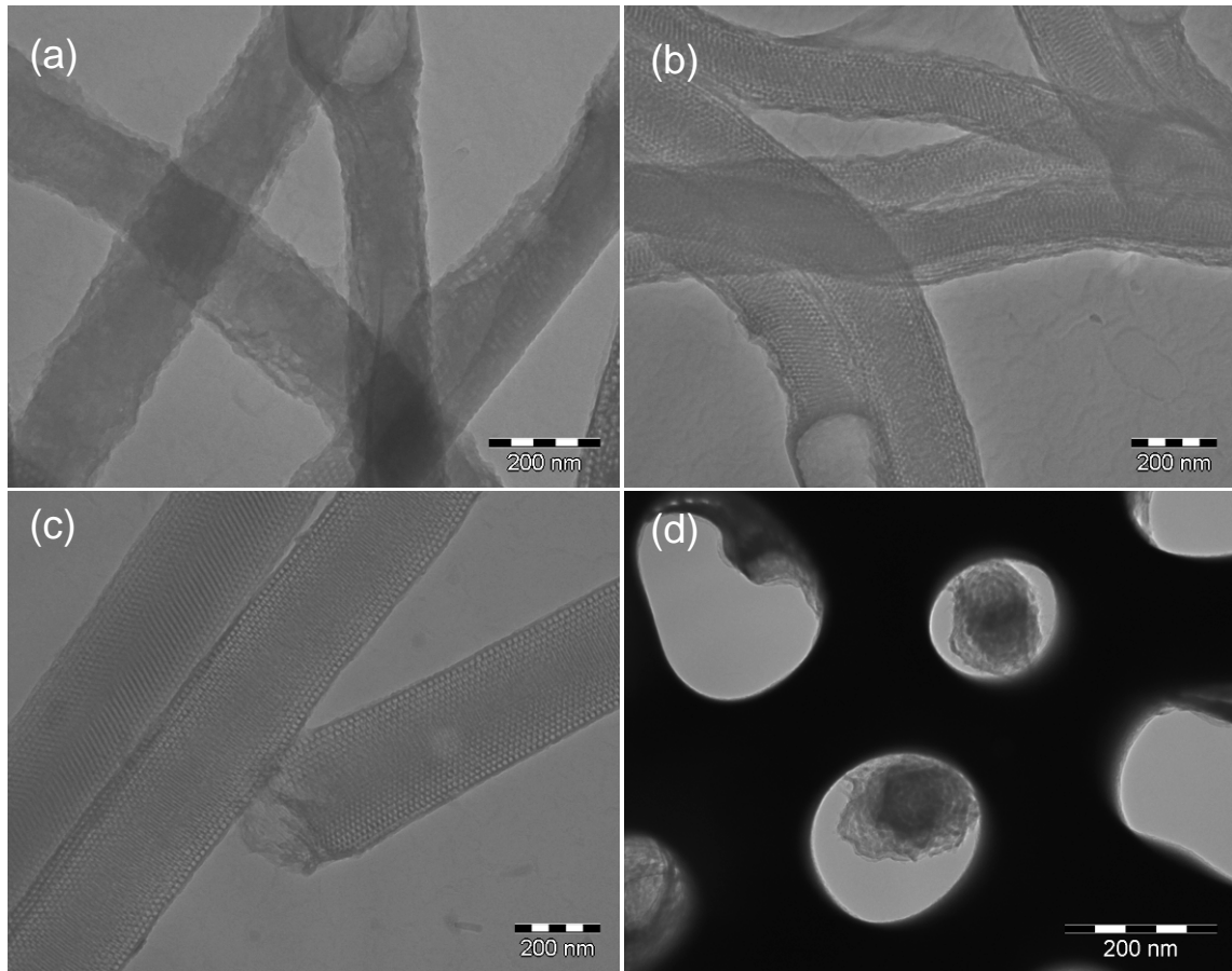
Figure 2. TEM images of the released carbon nanofibres prepared with (a) 0.07, (b) 0.1 and (c) 0.3 mL of the precursor sol and top-view of (a) embedded within the AAO pores.
