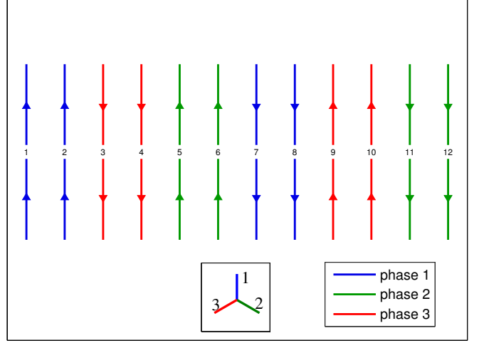
Figure 1. Example of plane scheme from which the Gorges polygon can be derived.
