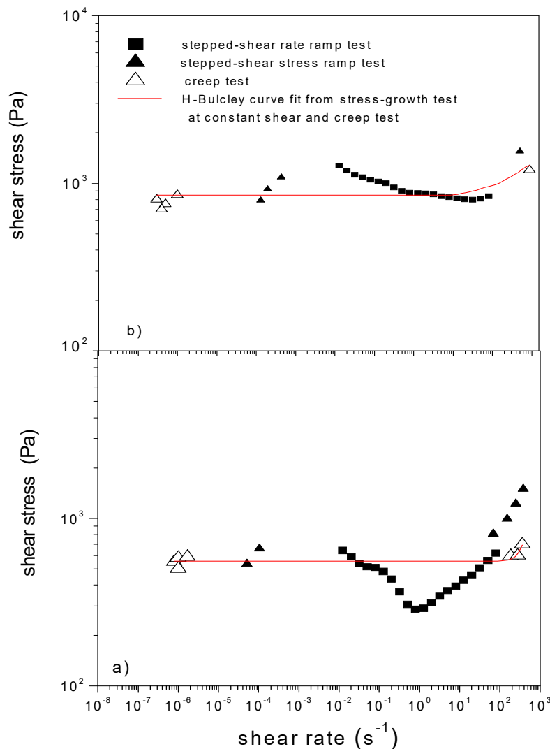
Figure 8. Steady-state flow curves obtained with different rheological tests and fitted to the Herschel-Bulkley model for calcium complex (a) and polyurea (b) greases.
