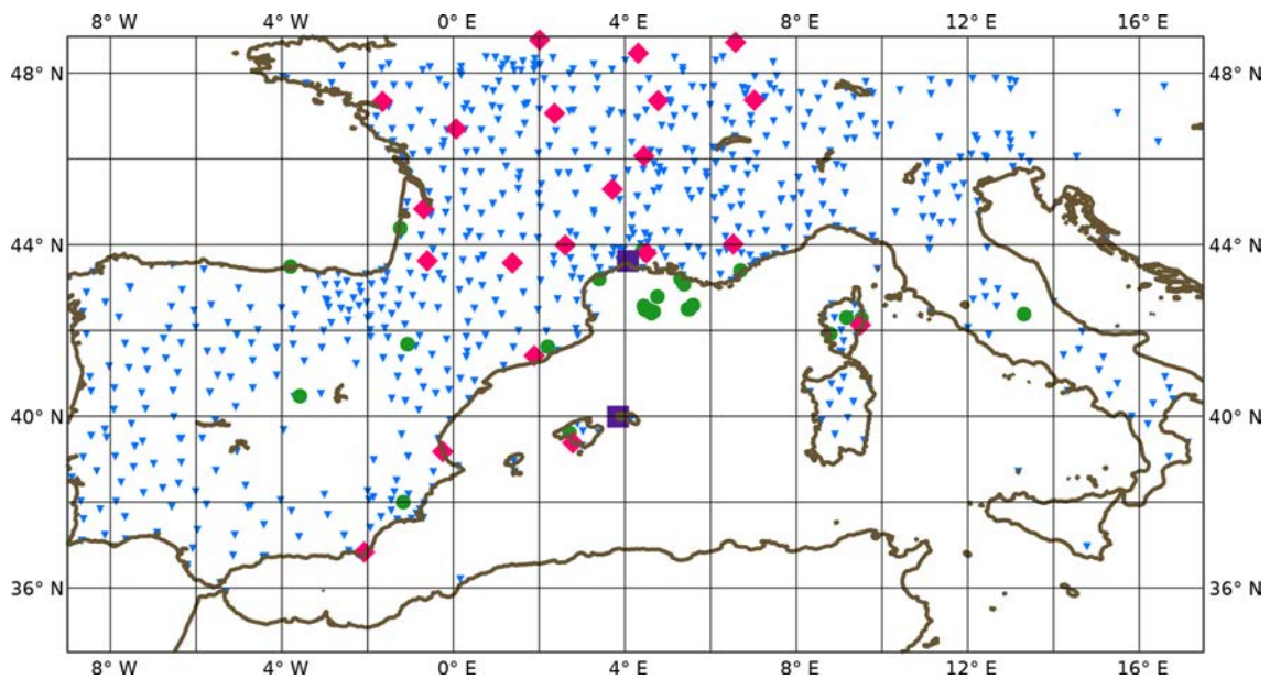
Figure 4. REANA2 assimilated data focus: green disks represent the location of radiosondes (fixed and mobile) taken into account at high resolution, red diamonds the position of the Doppler radars, violet squares the lidar sites, and blue triangles the global positioning system (GPS) and GNSS stations.
