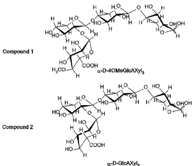
Figure 3. Compounds 1 and 2 produced from hemicellulose extract of C. cardunculus and ES-GTM endo-xyl.
