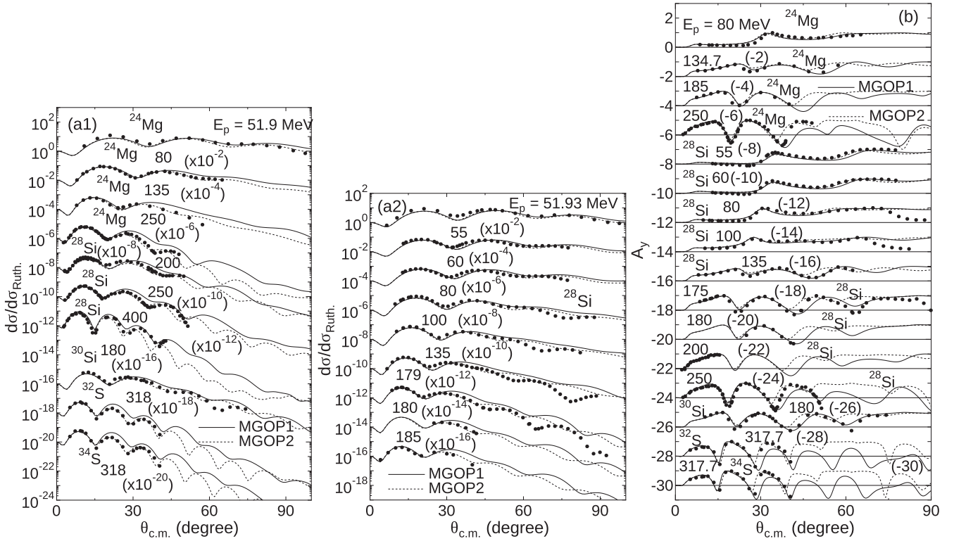
FIG. 19. (a) Elastic-scattering cross sections of p + ^{24}\text{Mg} , ^{28}\text{Si} , ^{30}\text{Si} , ^{32}\text{S} , and ^{34}\text{S} systems at E_p = 51.9 – 400 MeV in the Rutherford ratio and (b) analyzing power of p + ^{24}\text{Mg} , ^{28}\text{Si} , ^{30}\text{Si} , ^{32}\text{S} , and ^{34}\text{S} systems at E_p = 55 – 317.7 MeV. The experimental data are taken from Refs. [74,112,137,157–166].
