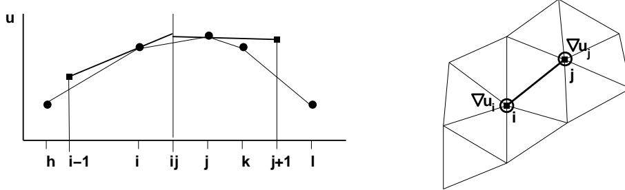
Figure 4 Higher Order Approximations
