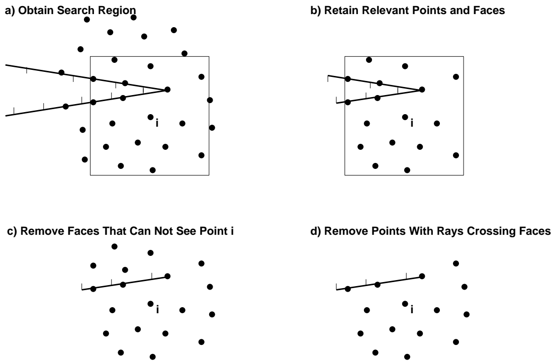
Figure 2 Search for Close Points
