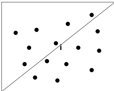
a) Place Points in Macro-Triangles
