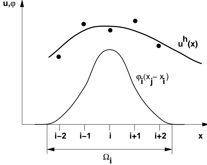
Figure 1 WLSQ Procedure
