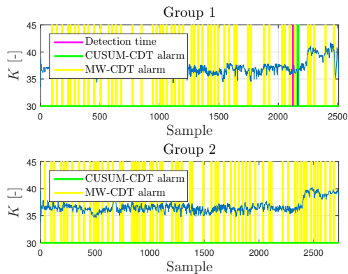
Fig. 9. K parameter monitoring alarms by the CUSUM-CDT technique.
