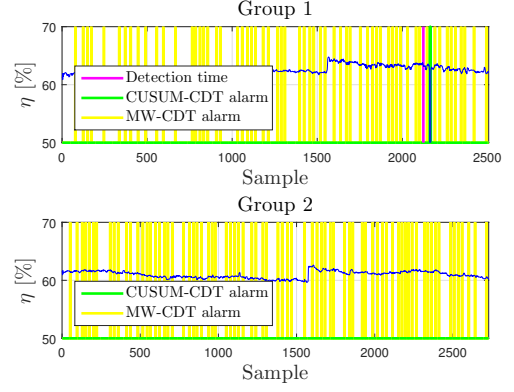
Fig. 7. Efficiency monitoring alarms by the CUSUM-CDT technique.
