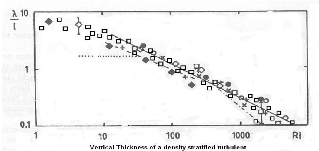
Figure 18. Non dimensional thickness of a density interface subject to oscillating grid turbulence on one side of the interface adapted from [16]. Different symbols correspond to different grid frecuencies
