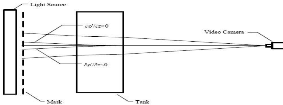
Figure 7. Detail of the synthetic schliering set up at DAMTP, Cambridge.
