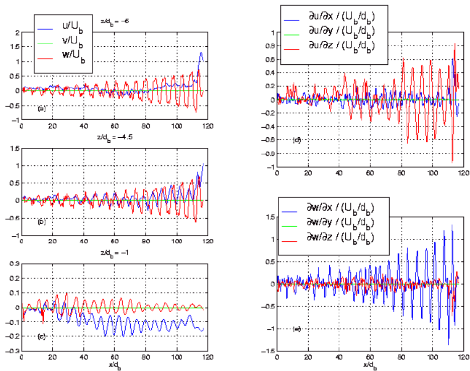
Fig. 4. Variations behind the single horizontal grid bar of the velocity and its spatial local derivatives, which indicate the structure of the wake, U_b = 4.4 cm/s is the mean bar velocity.
