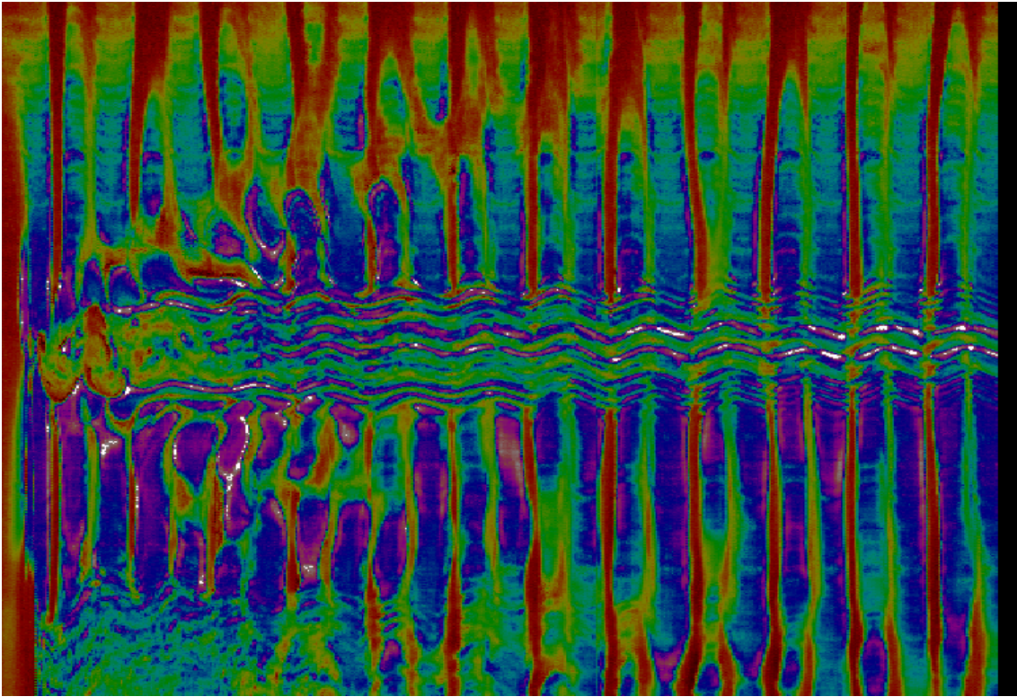
Figure 13.- Time series of a vertical line during 100 s at 50Hz of the passage of a horizontal bar in a linear stratification. Red and blue show the crests and troughs of the internal waves (density derivative)
