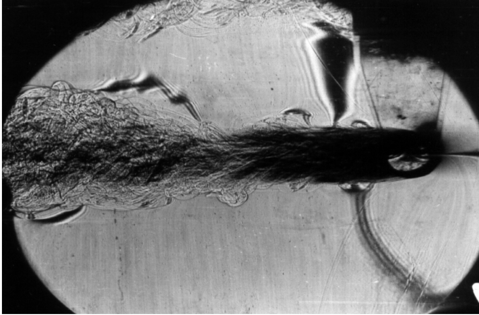
Figure 11. Image of the internal wave collapse in a very strongly stratified flow (Experiment performed at Moscow Institute of Problems in Mechanics)
