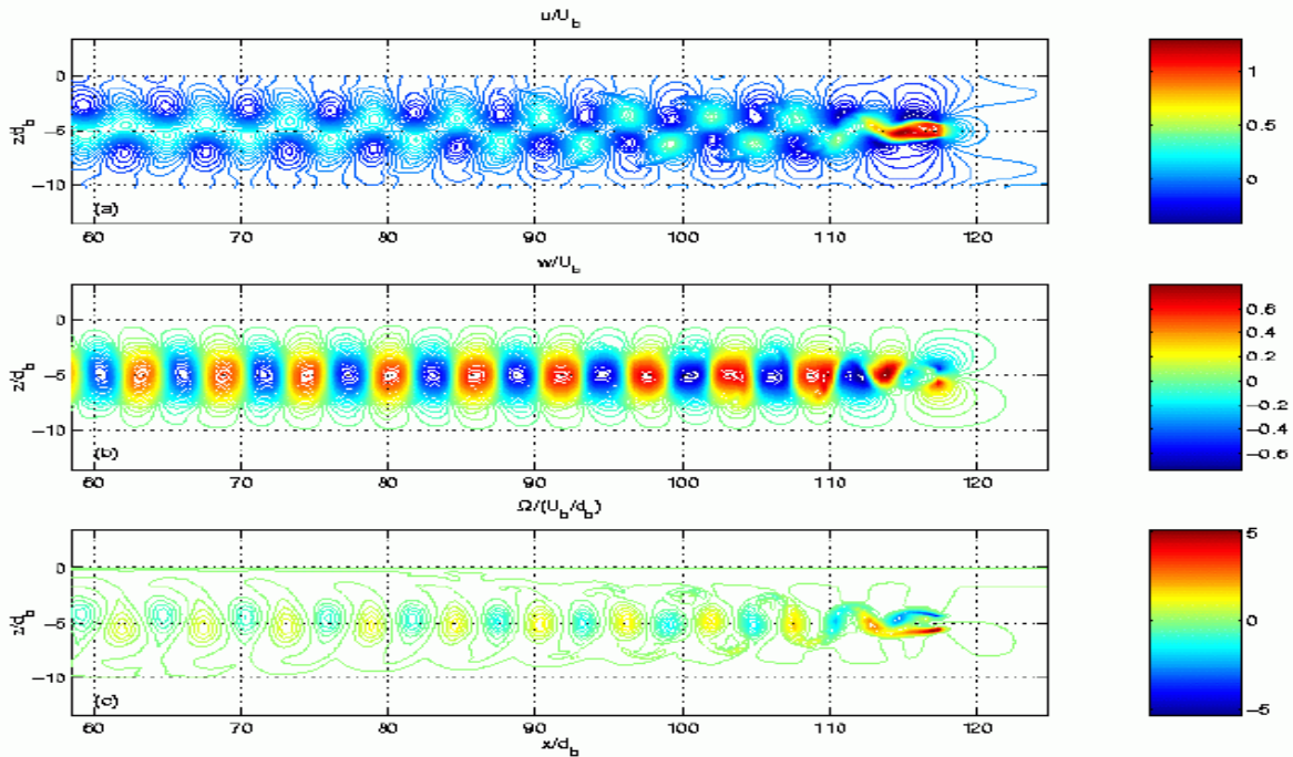
Fig. 2. Values of the horizontal and vertical velocities (above) as well as the sideways vorticity (below)
