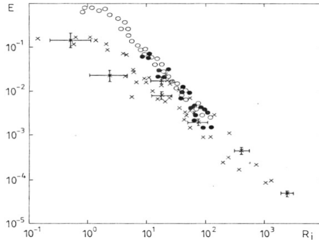
Figure 20. Direct measurements of entrainment as a function of the local Richardson number for these experiments the interface remains sharp. Open circles [35], closed circles [16], crosses [26] are experiments near a flat boundary.
