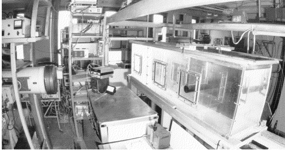
Figure 9. Large stratified tank used at IPM. at Moscow, described in [17,18,31] Experimental apparatus used for the internal wave measurements in this paper.
