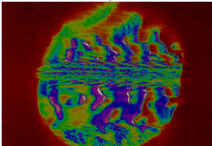
Figure 12. Sequence of Schlieren images of the flow visualization of the decay of the turbulence at a linear density interface. The collapsed inner region is clearly distinguished among the outer internal wave field
