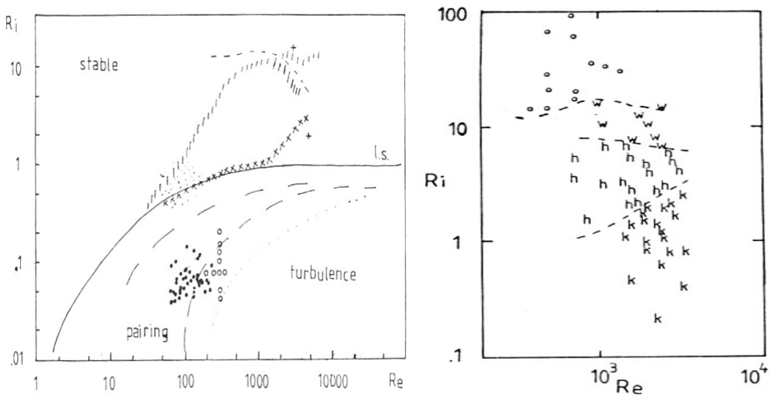
Figure 21.- Parameter space of a stratified non rotating flow from Redondo [10]. A general instability map with dots and circles as the experiments of [29,30] (left). Zoom of the right upper region of the parameter space ( Re, Ri ) where the symbols correspond to different dominant instabilities ( o – no turbulence; w – internal waves; h – Holmboe waves; k – Kelvin-Helmholtz billows (right)]
