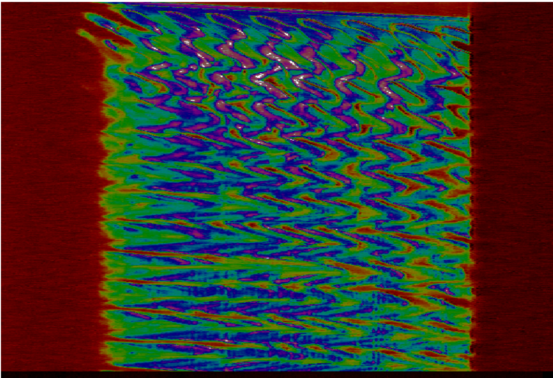
Figure 14. Time sequence (at 50 Hz) of Schlieren flow visualization of a horizontal line of the decay of the turbulence at a linear density stratification.
