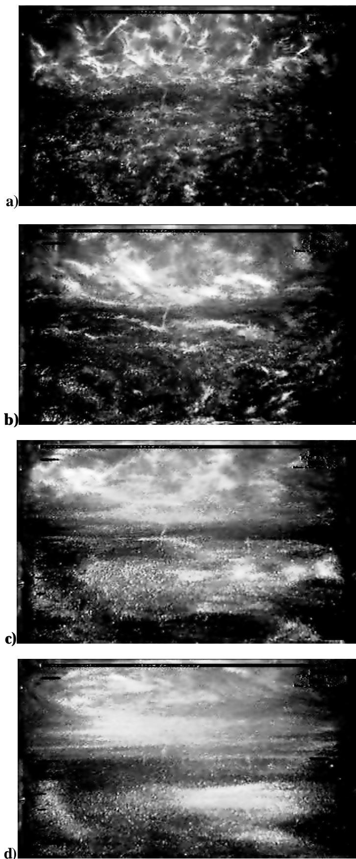
Figure 19. Pearlescence flow visualization of the decay of the turbulence at a sharp density interface. The collapse times measured in terms of the Brunt-Vaisalla frequency are a) N , b) 2N , c) 5N , d) 10N ; Ri = 30 .
