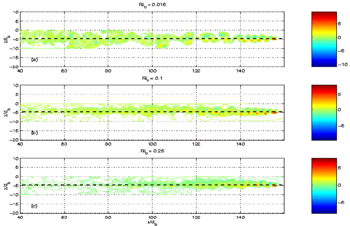
Fig. 3. Comparison of the spanwise vorticity in the wakes of three different numerical experiments with initial numbers Ri_b = 0.015 (top), Ri_b = 0.1 (centre), Ri_b = 0.25 (bottom), The Reynolds number is Re = 880 , The bar size is d_b = 2 cm, and its velocity U_b = 4.4 cm/s.
