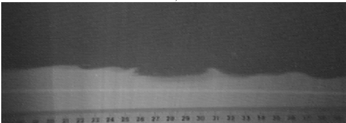
Figure 16. Laser Induced Fluorescence flow visualization of the effect of the shear generated turbulence at a sharp density interface. The intermediate Ri, Re of the experiment has the conditions for Holmboe instability development.
