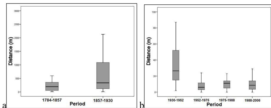
Fig. 6. Changes in the medians and quartiles (a) between the First and Second Military Survey, and (b) at the successive terms
