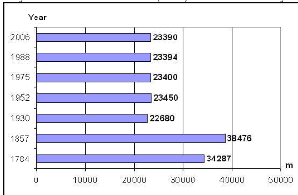
Fig. 5. The length changes of the studied reach of the River Bodrog between 1784 and 2006
