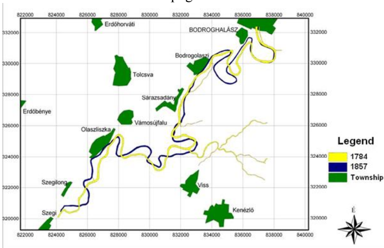
Fig. 4. The study area at the time of the First (1784) and Second Military Survey (1857)
