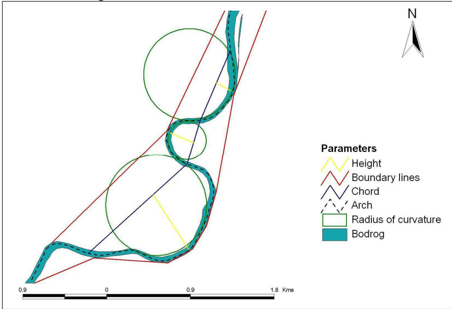
Fig. 3. The measured parameters based on the database of 1952
