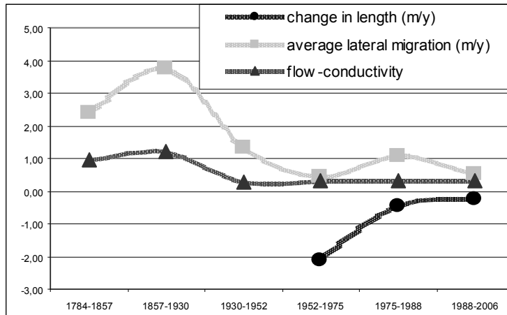
Fig. 7. The change of dynamic parameters of the river section
