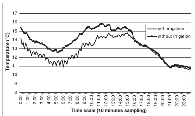
Figure 2: Effect of irrigation those days when the night temperature ( T > 10 °C) and wind speed (Average > 10 m/s) was high between March 15 and May 15, 2010
