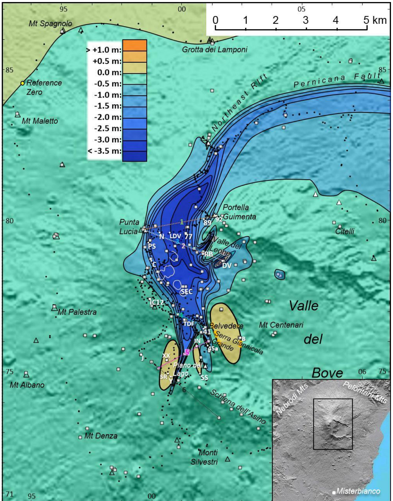
Fig. 1. Map showing contours of vertical ground deformation at Mt Etna during the 43 years August 1975 – September 2018. The reference zero is north of Monte Maletto at top left, 8 km northwest of the summit and 1850 metres below it. Black dots indicate levelling stations, white squares denote three-dimensional
