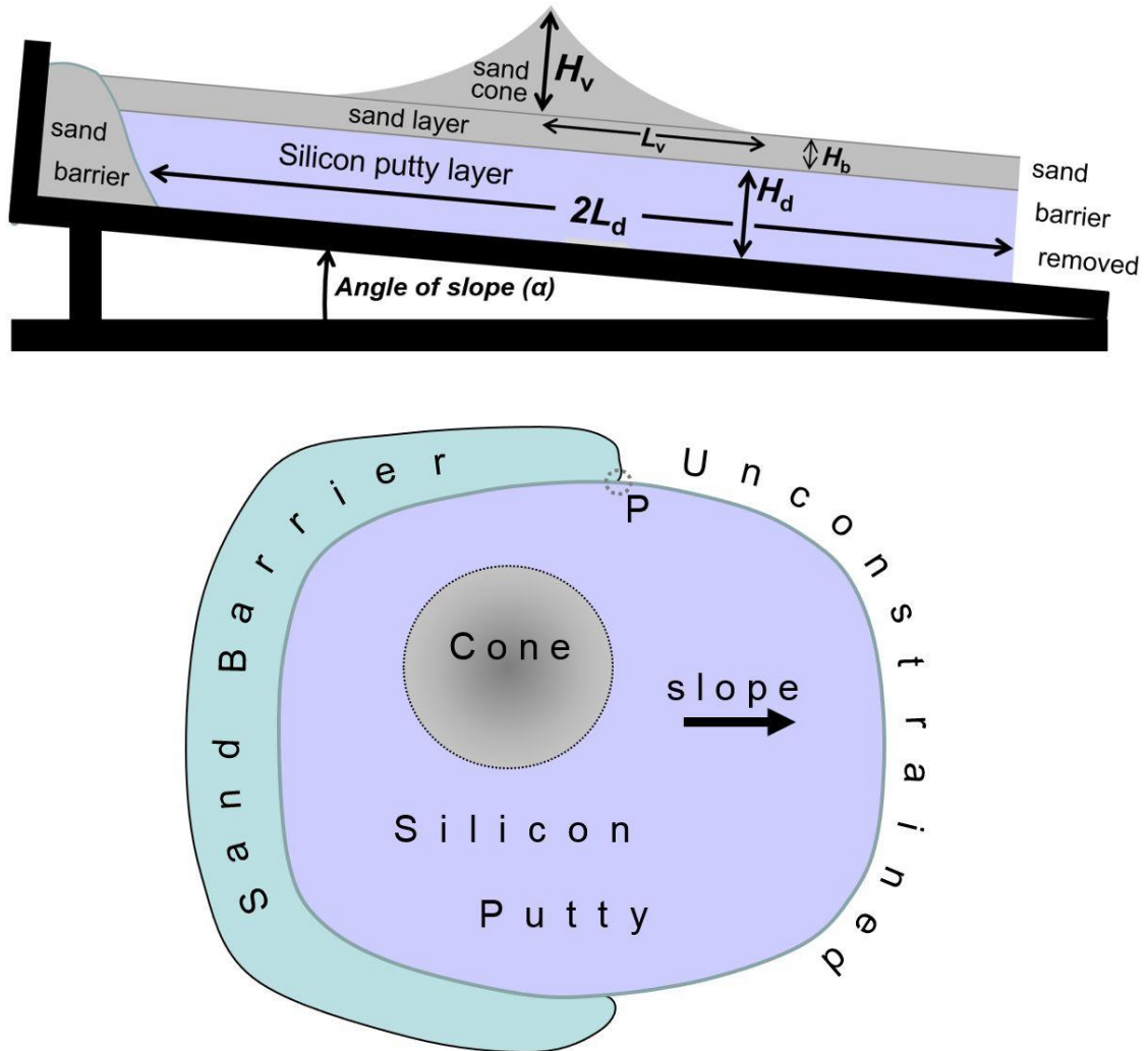
Fig. 5. Analogue model set-up showing cross section through apparatus (top) and plan view (bottom). In the plan view, the cone is placed asymmetrically upon the silicon putty to match the situation at Mt Etna (Fig. 1 inset) where the cone is closer to the Monte Peloritani to the north. Similarly the silicon putty extends further on the right side, to mimic the unconstrained slope on this side that continues beneath the Mediterranean Sea.
