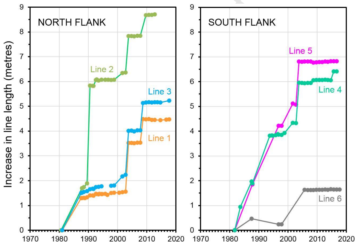
Fig. 4. Graben opening portrayed by increasing line length between stations east and west of the graben 1980 – 2018. Position of each line is shown in fig. 1. Values are from trilateration measurements 1981-1994, and dual-frequency GPS 1994-2018. The north flank values (lines 1, 2 & 3) for 1980 are derived from the 1980-81 displacement model in Bonaccorso (1999). The displacements 1980-1987 for these lines should be regarded as minimum values, as they do not include possible displacements during the 1983, 1985 and 1986-7 eruptions. Elastic modelling of these latter eruptions (Murray & Pullen 1984, Murray 1990) suggests that such displacements would be negligible for the 1983 and 1986-7 eruptions, but up to a possible 0.1 m for the 1985 eruption.
