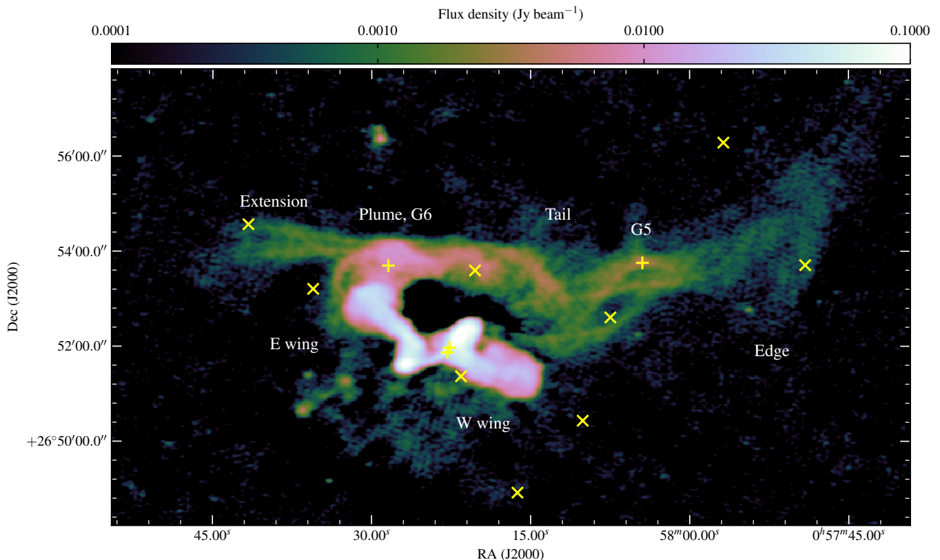
Figure 1. LOFAR colourscale of the radio emission from NGC 326. The colour scale is logarithmic over the range shown by the colour bar (in units of \text{Jy beam}^{-1} for the resolution of 8.2 \times 5.1 arcsec). yellow crosses mark the positions of potential cluster members; + signs are those in the spectroscopic study of Werner et al. (1999) and × signs show candidate galaxies selected from NED as described in the text. The double nuclei of NGC 326 are represented by the two adjacent crosses close to the centre of the image. Features referred to in the text are labelled.
