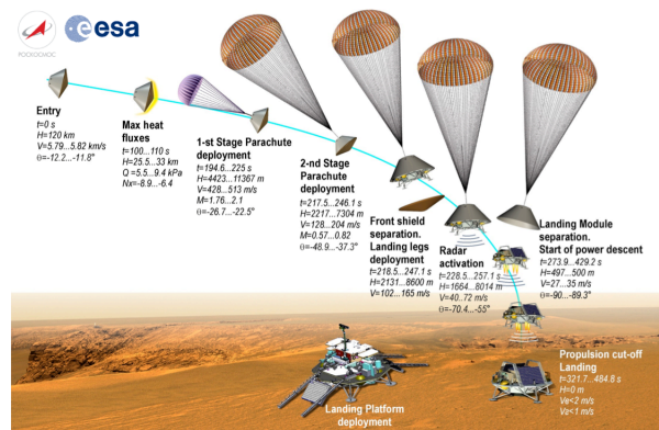
Figure 1: ExoMars 2020 EDL scenario
