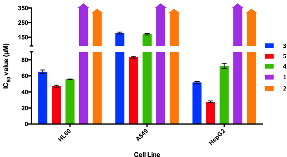
Figure 4. Summary of the IC_{50} values obtained for the specified compounds in the human cancer cell lines: HL-60, A549 and HepG2 cells. IC_{50} values for compounds 1 and 2 were not determined due to solubility limitations but were greater than 300 \mu\text{M} (as indicated by column arrow). Each column represents the average IC_{50} value determined from triplicate MTT assays.
