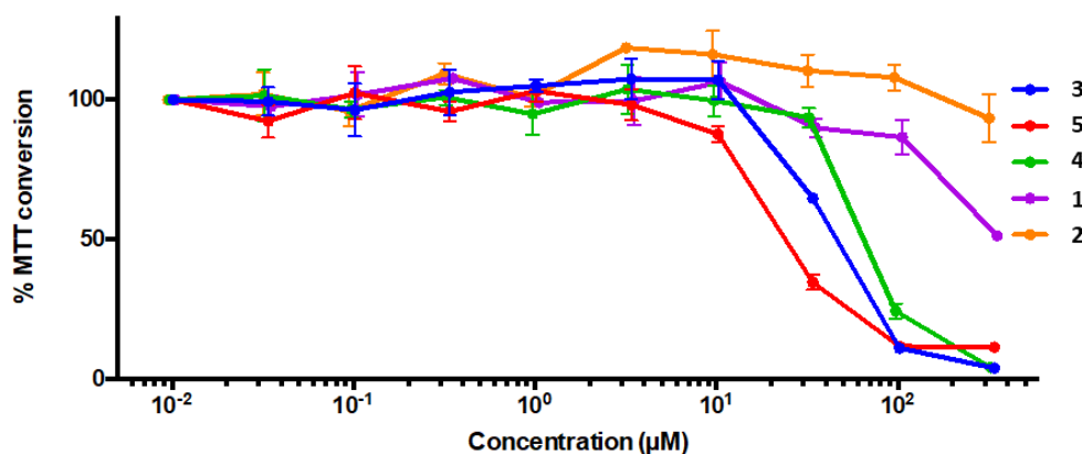
Figure 3. The concentration response curves for the specified compounds in the human suspension cancer cell line (HL-60 leukemia cells, (A)) and the human fibroblastic cancer cell lines (A549 lung cancer cells (B) and HepG2 liver cancer cells (C)).
