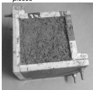
Figure 8. The mixture is properly compacted into the mould
