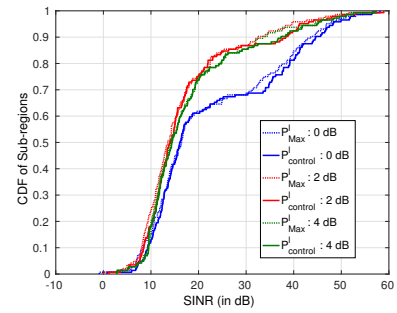
Figure 17: SINR CDF with maximum and controlled powers.
