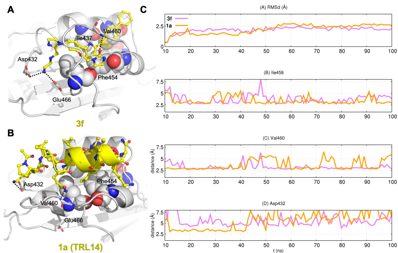
Figure 3. Comparative results from molecular dynamics (MD) simulations of Li-TryR:1a and Li-TryR:3f complexes. (A) Representative structure of 3f (shown as sticks and balls; C atoms colored in yellow) bound at the dimerization interface of a Li-TryR monomer (C atoms colored in grey). (B) Representative structure of the complex formed between a Li-TryR monomer and peptide 1a (TRL14) ( 1a ) with a Lys at position 2 (PKIIQSVGICMKM, C atoms colored in yellow). (C) Evolution of the root-mean-square deviation (RMSd, Å) of bound 3f or 1a (top) and time evolution of the distances (Å) separating 3f from the backbone oxygen of Ile458, backbone nitrogen of Val460 (middle) and the carboxylate oxygen of Asp432 (bottom) along 100 ns of unrestrained MD simulation.
