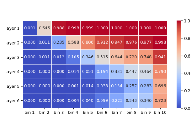
Figure 14: Frequency-based classification accuracy on states from the EN→RU decoder.
